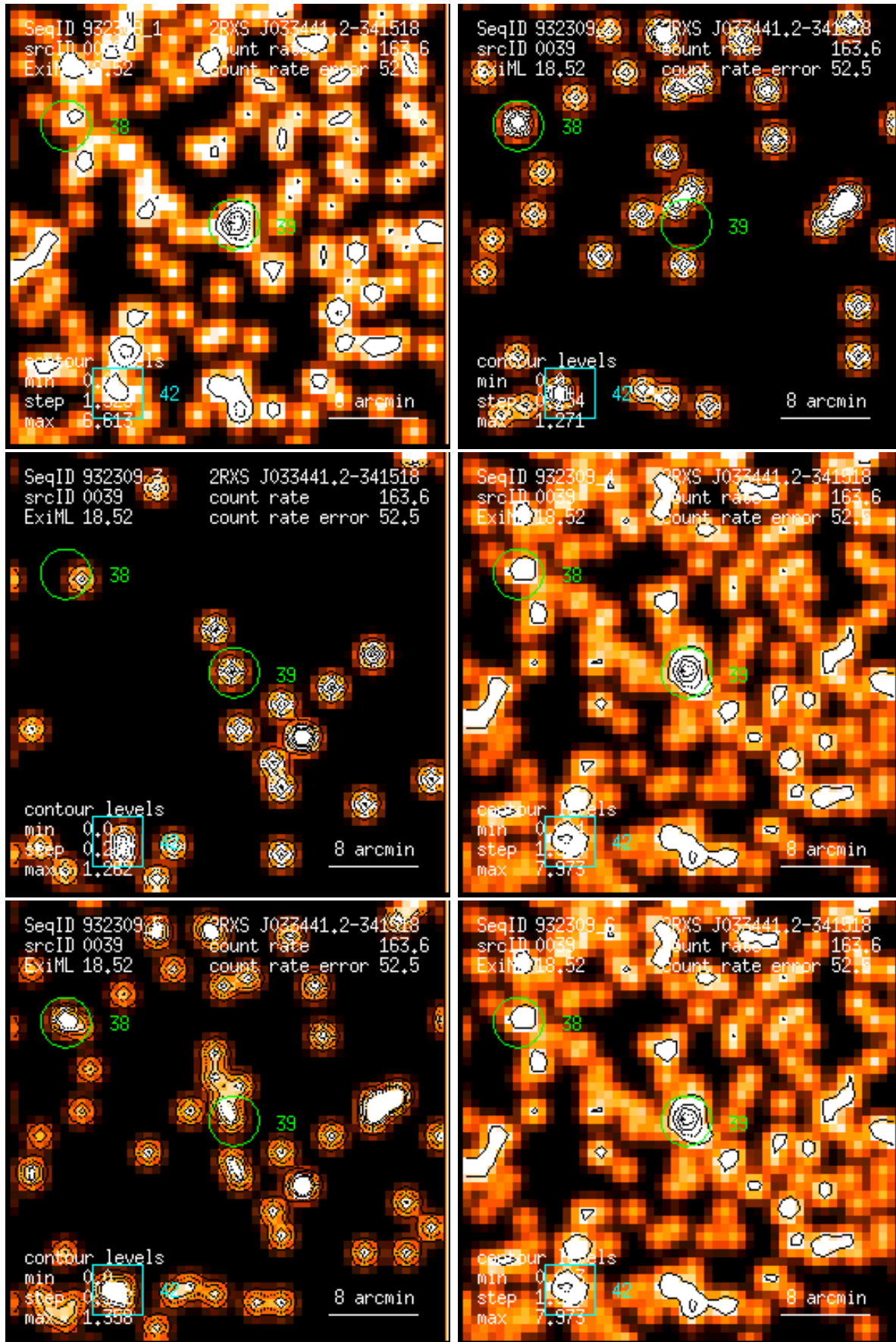
Figure 39: RASS 932309: detection 0039: band rate images, Gaussian filter: (1) PSPC channels 11 – 41, (2) 52 – 90, (3) 91 – 201, (4) 11 – 235, (5) 52 – 201, (6) 11 – 201. Broad band rates in counts/ks. Band rate contour levels in counts/ks/arcmin 2 .
