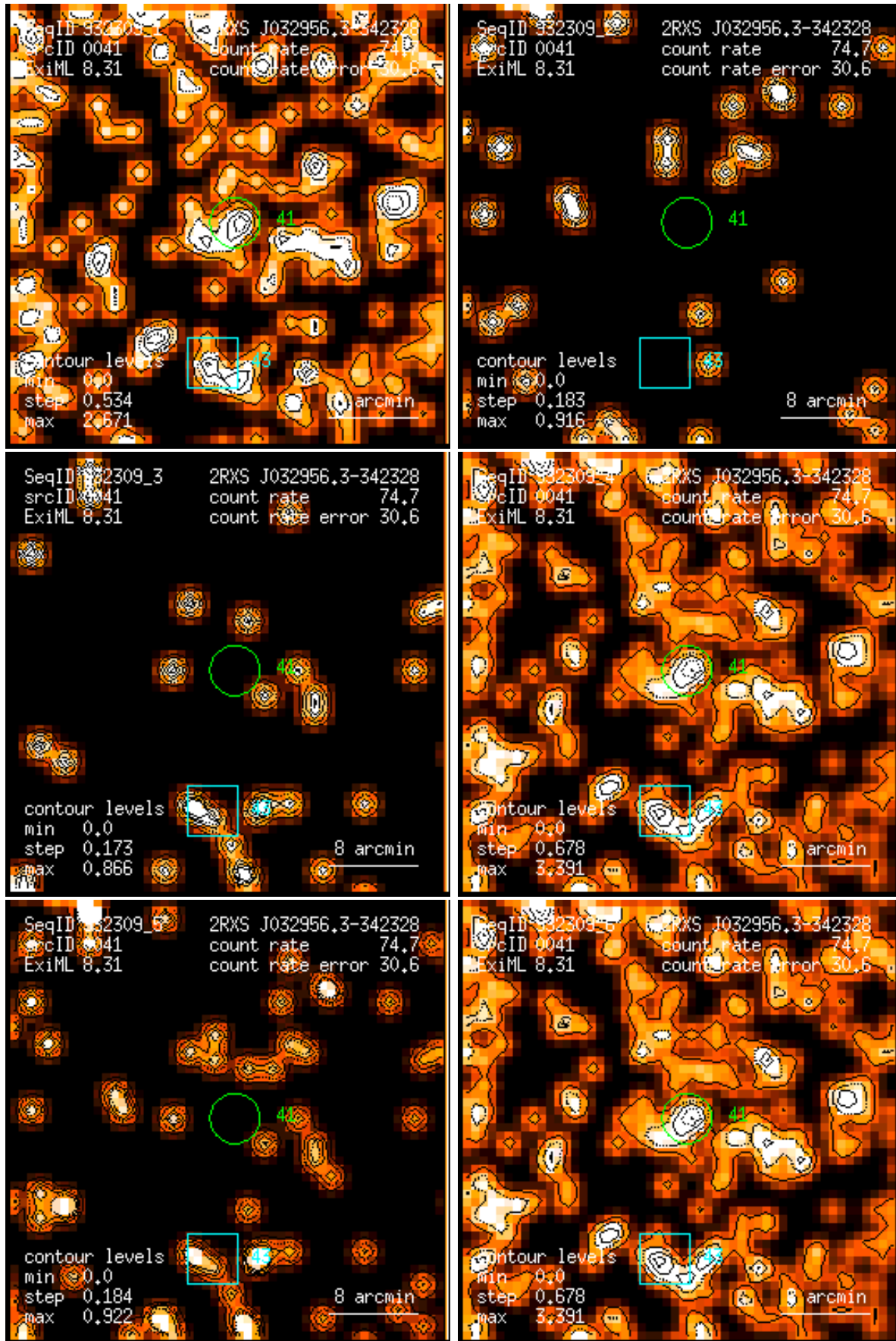
Figure 41: RASS 932309: detection 0041: band rate images, Gaussian filter: (1) PSPC channels 11 – 41, (2) 52 – 90, (3) 91 – 201, (4) 11 – 235, (5) 52 – 201, (6) 11 – 201. Broad band rates in counts/ks. Band rate contour levels in counts/ks/arcmin 2 .
