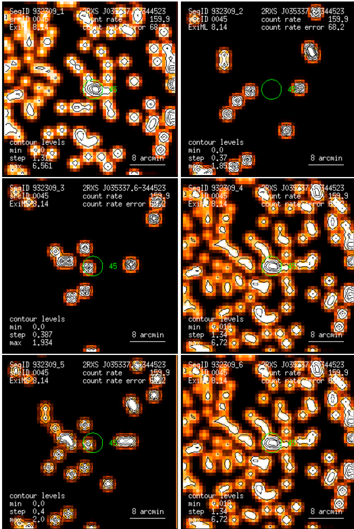
Figure 45: RASS 932309: detection 0045: band rate images, Gaussian filter: (1) PSPC channels 11 – 41, (2) 52 – 90, (3) 91 – 201, (4) 11 – 235, (5) 52 – 201, (6) 11 – 201. Broad band rates in counts/ks. Band rate contour levels in counts/ks/arcmin 2 .
