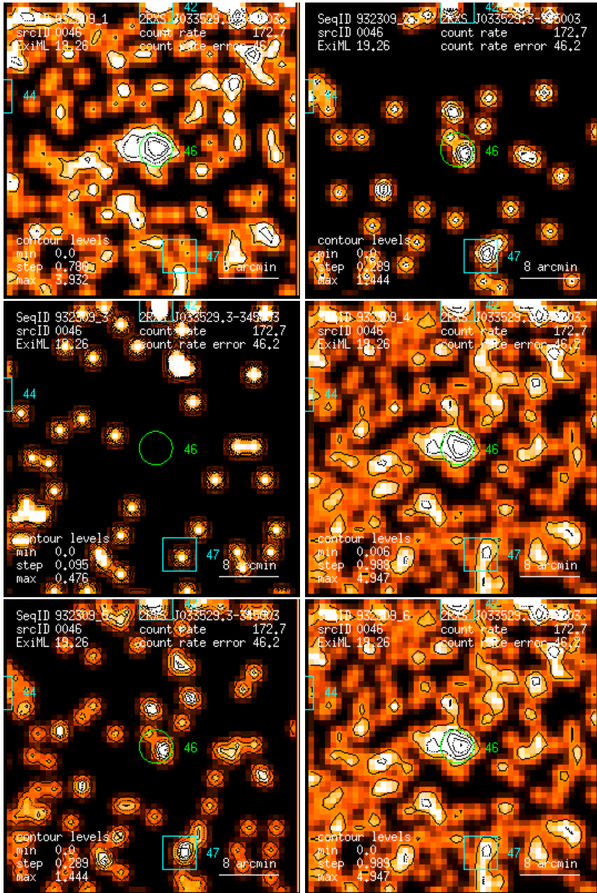
Figure 46: RASS 932309: detection 0046: band rate images, Gaussian filter: (1) PSPC channels 11 – 41, (2) 52 – 90, (3) 91 – 201, (4) 11 – 235, (5) 52 – 201, (6) 11 – 201. Broad band rates in counts/ks. Band rate contour levels in counts/ks/arcmin 2 .
