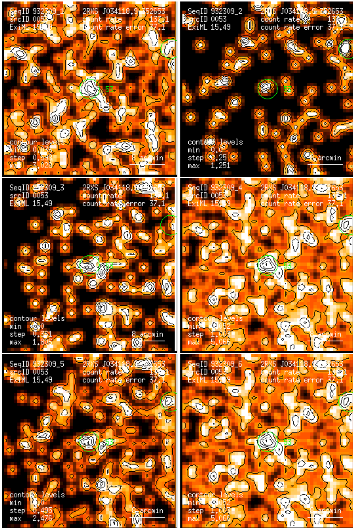
Figure 53: RASS 932309: detection 0053: band rate images, Gaussian filter: (1) PSPC channels 11 – 41, (2) 52 – 90, (3) 91 – 201, (4) 11 – 235, (5) 52 – 201, (6) 11 – 201. Broad band rates in counts/ks. Band rate contour levels in counts/ks/arcmin 2 .
