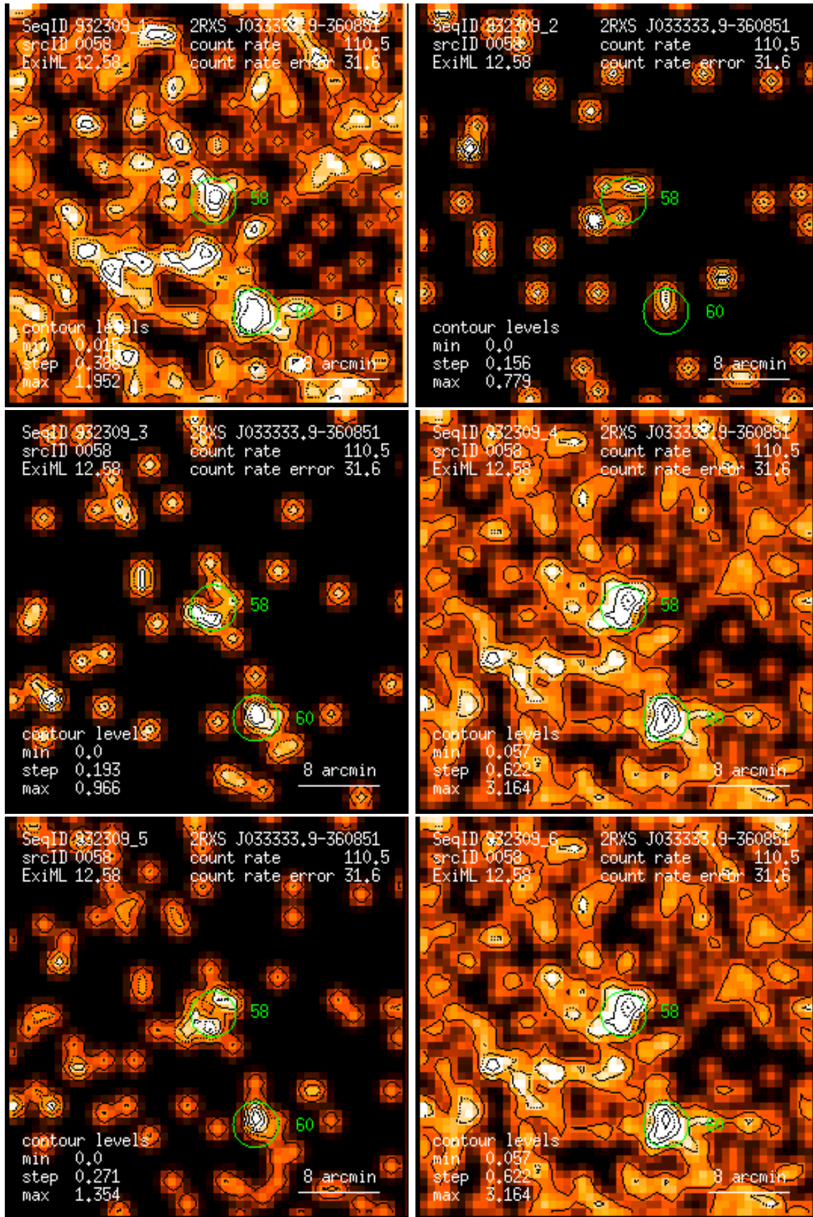
Figure 58: RASS 932309: detection 0058: band rate images, Gaussian filter: (1) PSPC channels 11 – 41, (2) 52 – 90, (3) 91 – 201, (4) 11 – 235, (5) 52 – 201, (6) 11 – 201. Broad band rates in counts/ks. Band rate contour levels in counts/ks/arcmin 2 .
