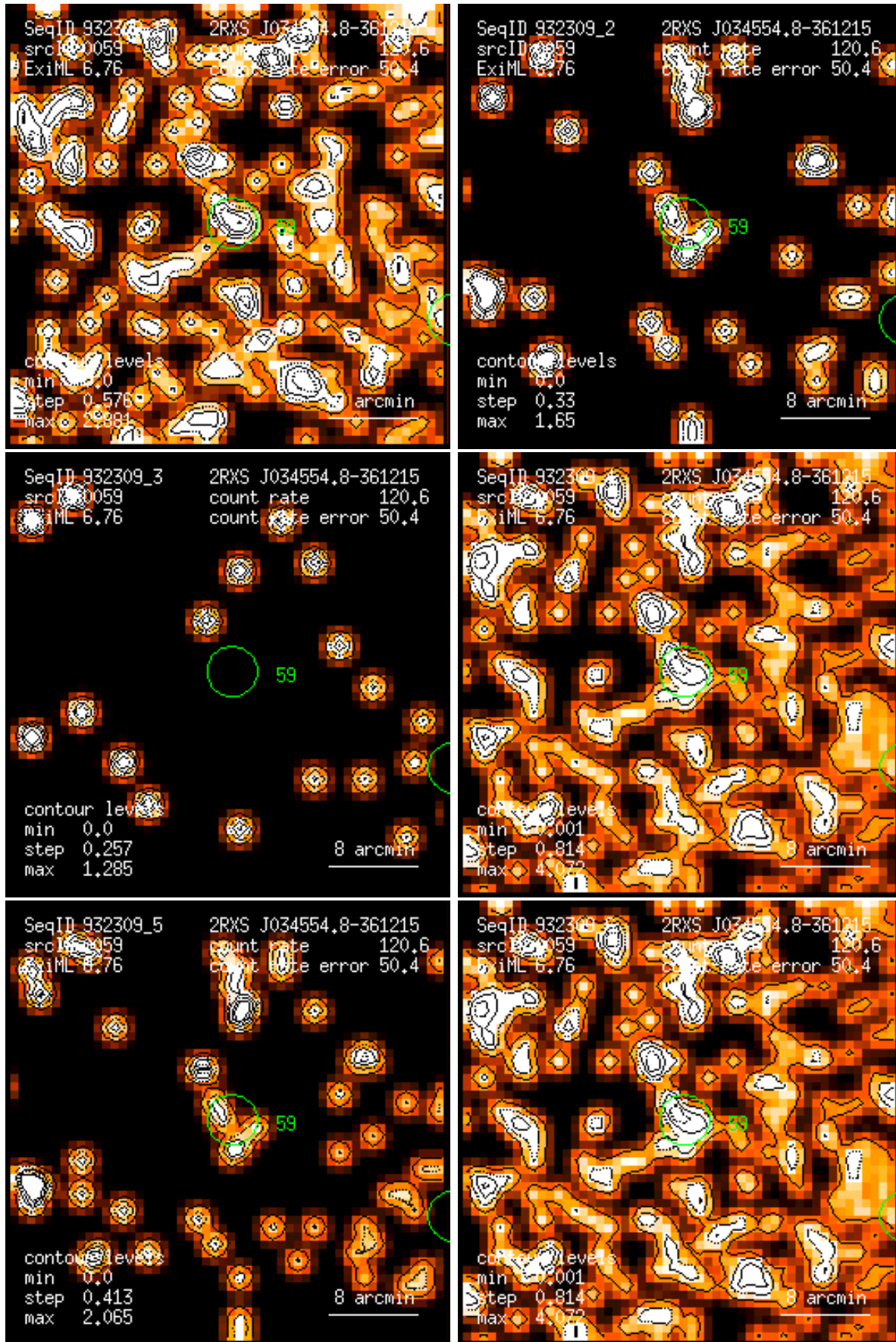
Figure 59: RASS 932309: detection 0059: band rate images, Gaussian filter: (1) PSPC channels 11 – 41, (2) 52 – 90, (3) 91 – 201, (4) 11 – 235, (5) 52 – 201, (6) 11 – 201. Broad band rates in counts/ks. Band rate contour levels in counts/ks/arcmin 2 .
