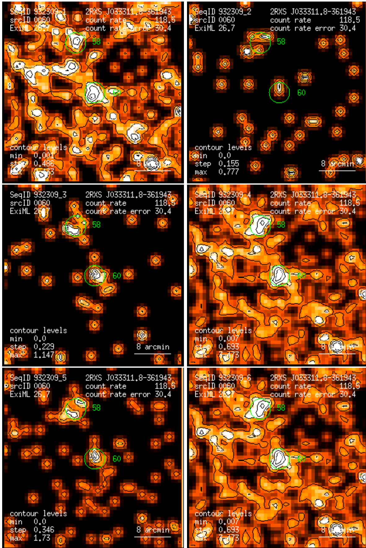
Figure 60: RASS 932309: detection 0060: band rate images, Gaussian filter: (1) PSPC channels 11 – 41, (2) 52 – 90, (3) 91 – 201, (4) 11 – 235, (5) 52 – 201, (6) 11 – 201. Broad band rates in counts/ks. Band rate contour levels in counts/ks/arcmin 2 .
