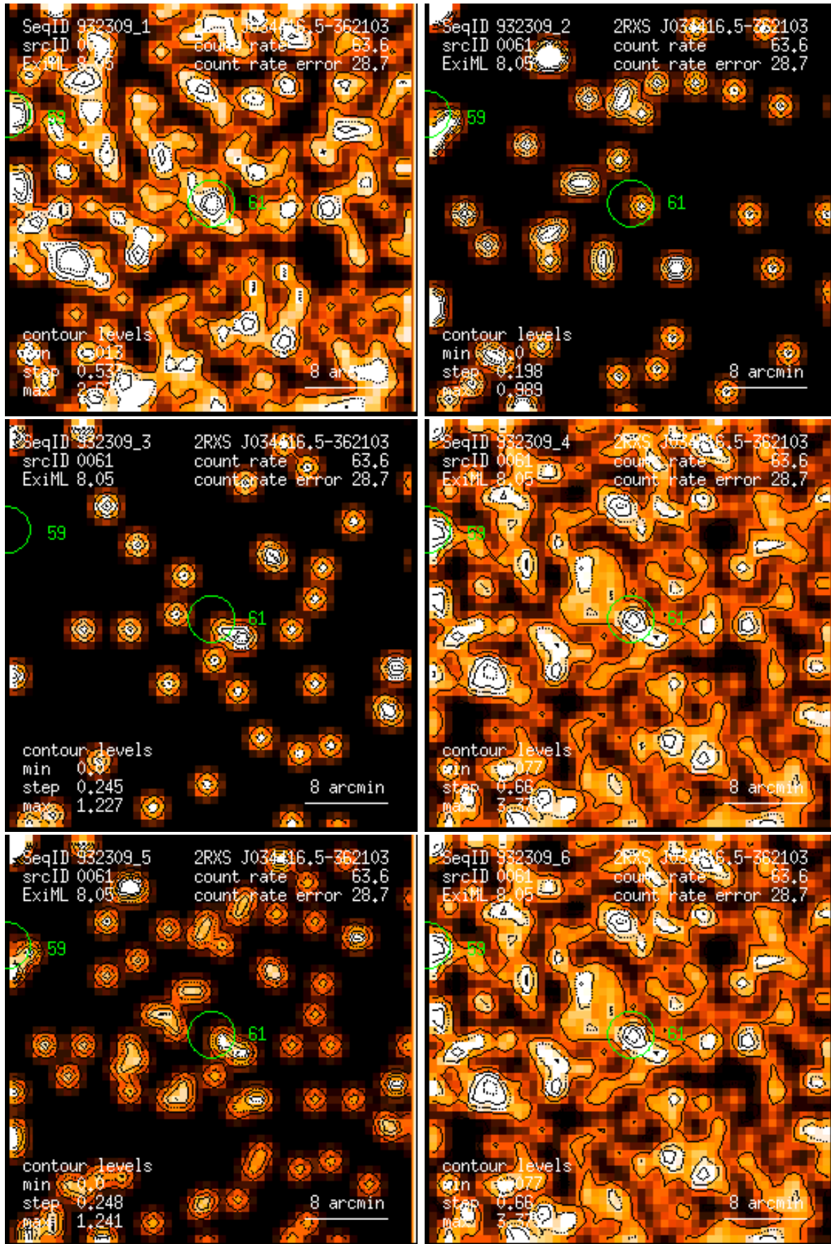
Figure 61: RASS 932309: detection 0061: band rate images, Gaussian filter: (1) PSPC channels 11 – 41, (2) 52 – 90, (3) 91 – 201, (4) 11 – 235, (5) 52 – 201, (6) 11 – 201. Broad band rates in counts/ks. Band rate contour levels in counts/ks/arcmin 2 .
