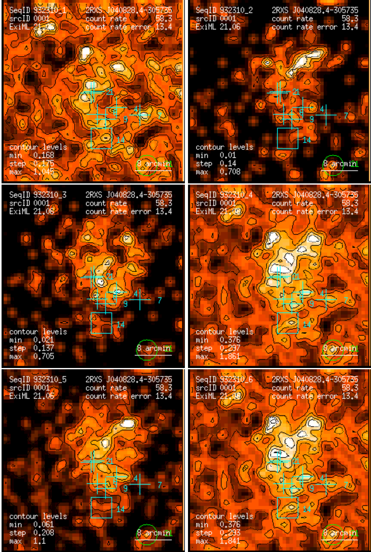
Figure 1: RASS 932310: detection 0001: band rate images, Gaussian filter: (1) PSPC channels 11 – 41, (2) 52 – 90, (3) 91 – 201, (4) 11 – 235, (5) 52 – 201, (6) 11 – 201. Broad band rates in counts/ks. Band rate contour levels in counts/ks/arcmin 2 .
