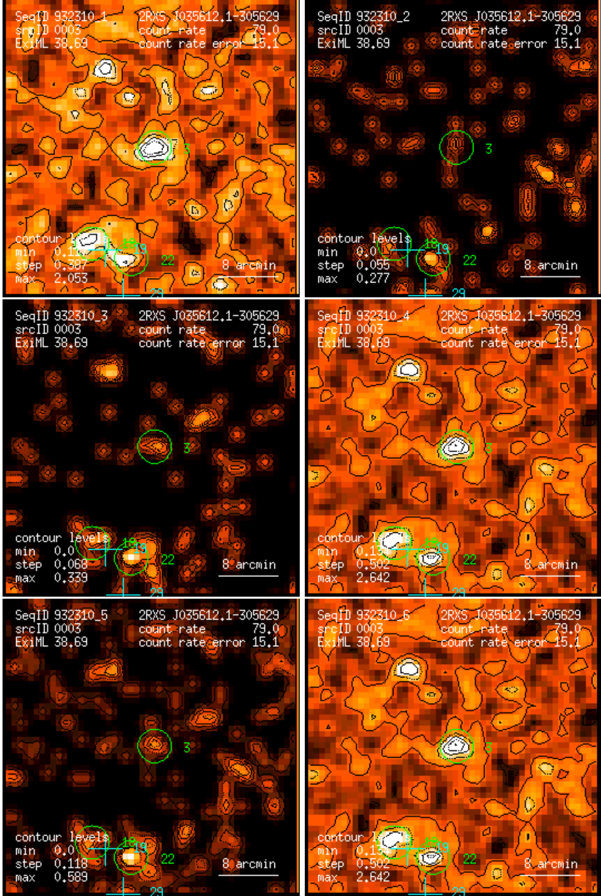
Figure 3: RASS 932310: detection 0003: band rate images, Gaussian filter: (1) PSPC channels 11 – 41, (2) 52 – 90, (3) 91 – 201, (4) 11 – 235, (5) 52 – 201, (6) 11 – 201. Broad band rates in counts/ks. Band rate contour levels in counts/ks/arcmin 2 .
