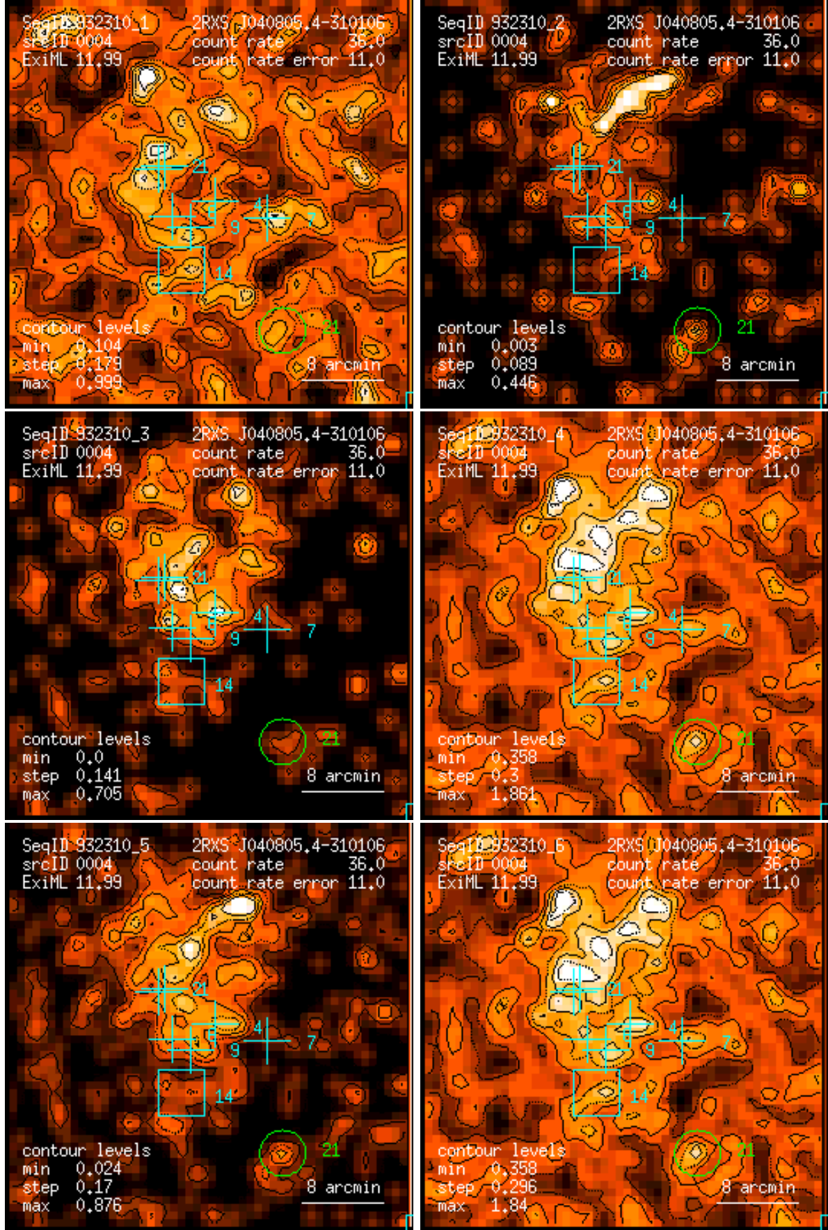
Figure 4: RASS 932310: detection 0004: band rate images, Gaussian filter: (1) PSPC channels 11 – 41, (2) 52 – 90, (3) 91 – 201, (4) 11 – 235, (5) 52 – 201, (6) 11 – 201. Broad band rates in counts/ks. Band rate contour levels in counts/ks/arcmin 2 .
