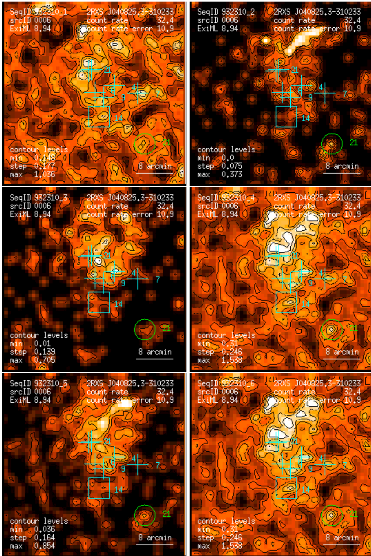
Figure 6: RASS 932310: detection 0006: band rate images, Gaussian filter: (1) PSPC channels 11 – 41, (2) 52 – 90, (3) 91 – 201, (4) 11 – 235, (5) 52 – 201, (6) 11 – 201. Broad band rates in counts/ks. Band rate contour levels in counts/ks/arcmin 2 .
