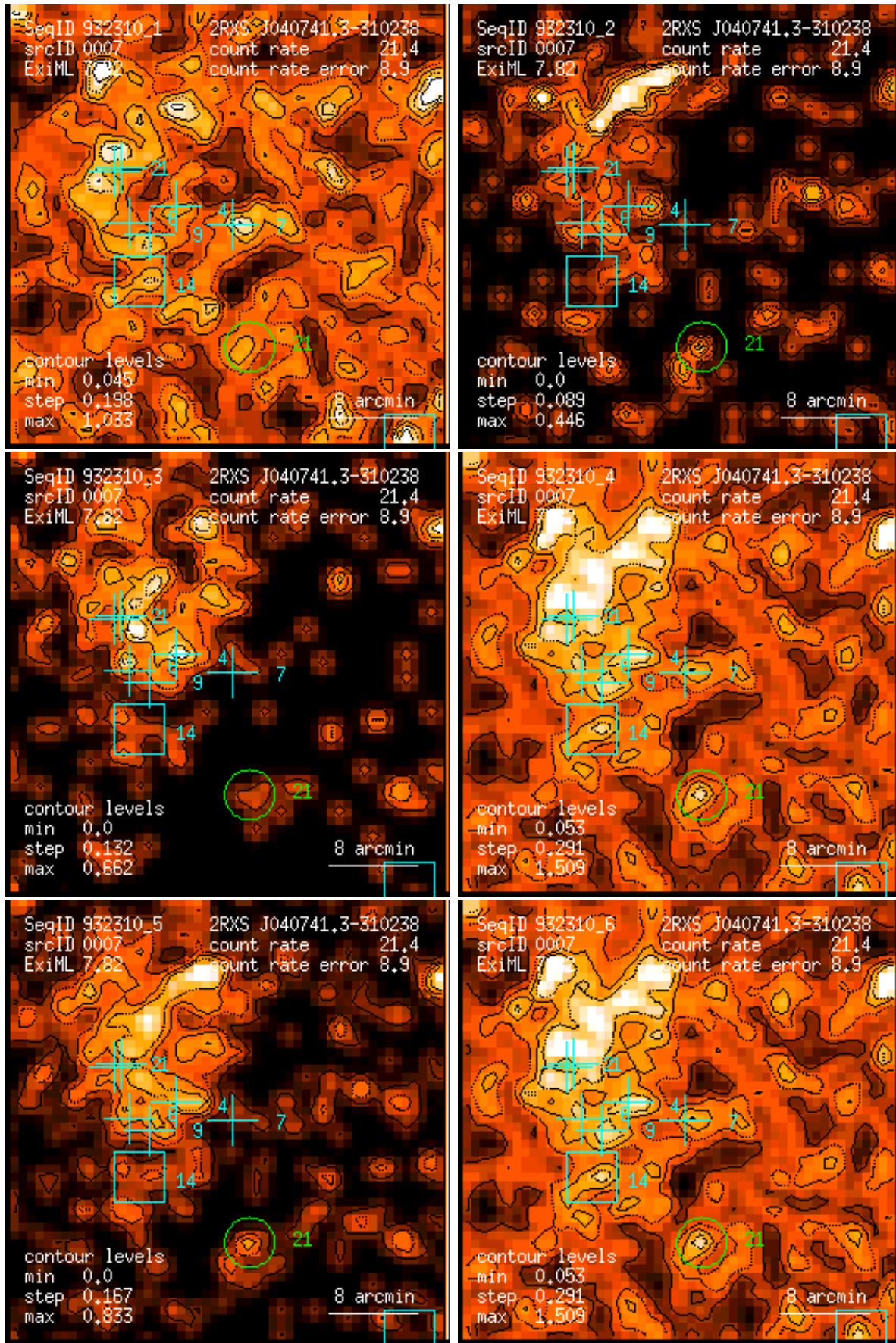
Figure 7: RASS 932310: detection 0007: band rate images, Gaussian filter: (1) PSPC channels 11 – 41, (2) 52 – 90, (3) 91 – 201, (4) 11 – 235, (5) 52 – 201, (6) 11 – 201. Broad band rates in counts/ks. Band rate contour levels in counts/ks/arcmin 2 .
