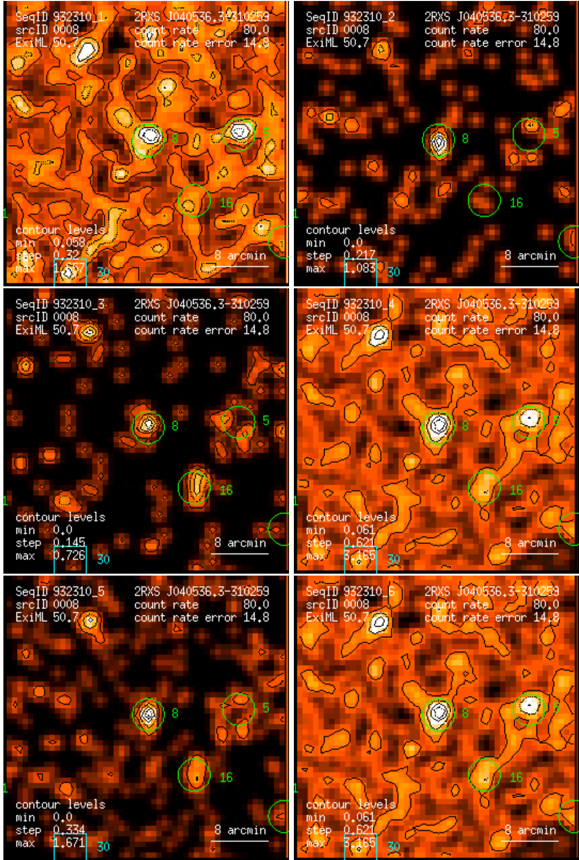
Figure 8: RASS 932310: detection 0008: band rate images, Gaussian filter: (1) PSPC channels 11 – 41, (2) 52 – 90, (3) 91 – 201, (4) 11 – 235, (5) 52 – 201, (6) 11 – 201. Broad band rates in counts/ks. Band rate contour levels in counts/ks/arcmin 2 .
