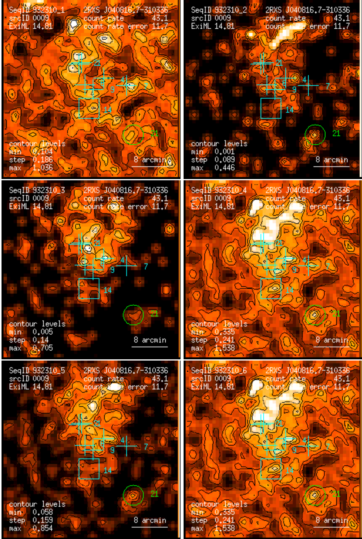
Figure 9: RASS 932310: detection 0009: band rate images, Gaussian filter: (1) PSPC channels 11 – 41, (2) 52 – 90, (3) 91 – 201, (4) 11 – 235, (5) 52 – 201, (6) 11 – 201. Broad band rates in counts/ks. Band rate contour levels in counts/ks/arcmin 2 .
