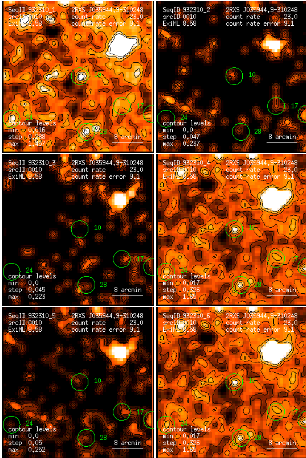
Figure 10: RASS 932310: detection 0010: band rate images, Gaussian filter: (1) PSPC channels 11 – 41, (2) 52 – 90, (3) 91 – 201, (4) 11 – 235, (5) 52 – 201, (6) 11 – 201. Broad band rates in counts/ks. Band rate contour levels in counts/ks/arcmin 2 .
