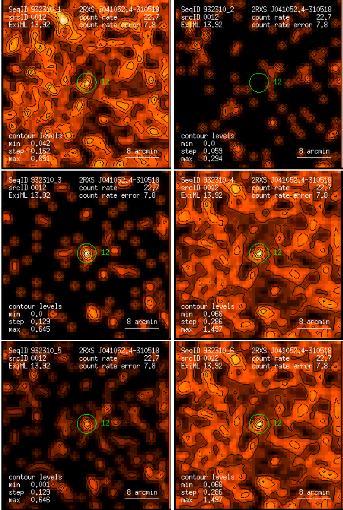
Figure 12: RASS 932310: detection 0012: band rate images, Gaussian filter: (1) PSPC channels 11 – 41, (2) 52 – 90, (3) 91 – 201, (4) 11 – 235, (5) 52 – 201, (6) 11 – 201. Broad band rates in counts/ks. Band rate contour levels in counts/ks/arcmin 2 .
