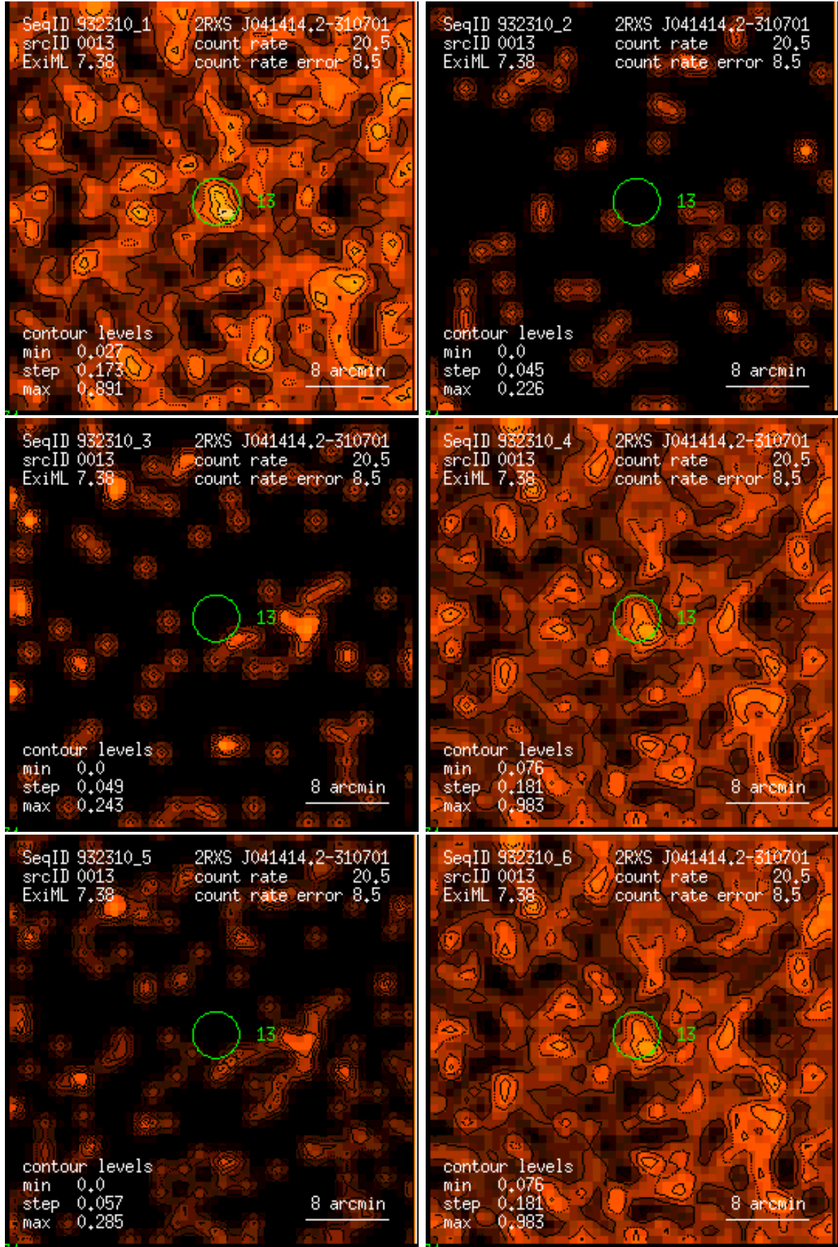
Figure 13: RASS 932310: detection 0013: band rate images, Gaussian filter: (1) PSPC channels 11 – 41, (2) 52 – 90, (3) 91 – 201, (4) 11 – 235, (5) 52 – 201, (6) 11 – 201. Broad band rates in counts/ks. Band rate contour levels in counts/ks/arcmin 2 .
