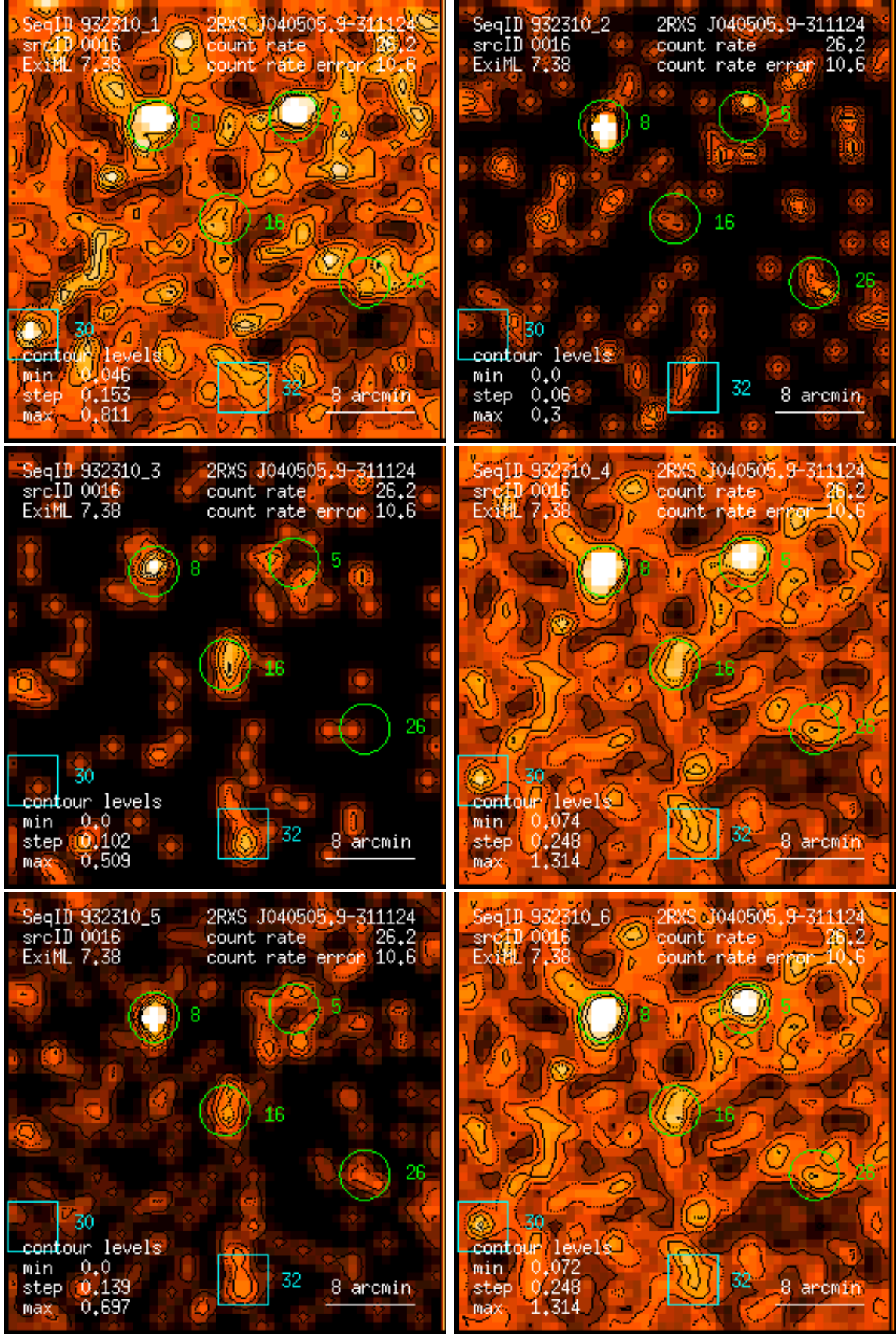
Figure 16: RASS 932310: detection 0016: band rate images, Gaussian filter: (1) PSPC channels 11 – 41, (2) 52 – 90, (3) 91 – 201, (4) 11 – 235, (5) 52 – 201, (6) 11 – 201. Broad band rates in counts/ks. Band rate contour levels in counts/ks/arcmin 2 .
