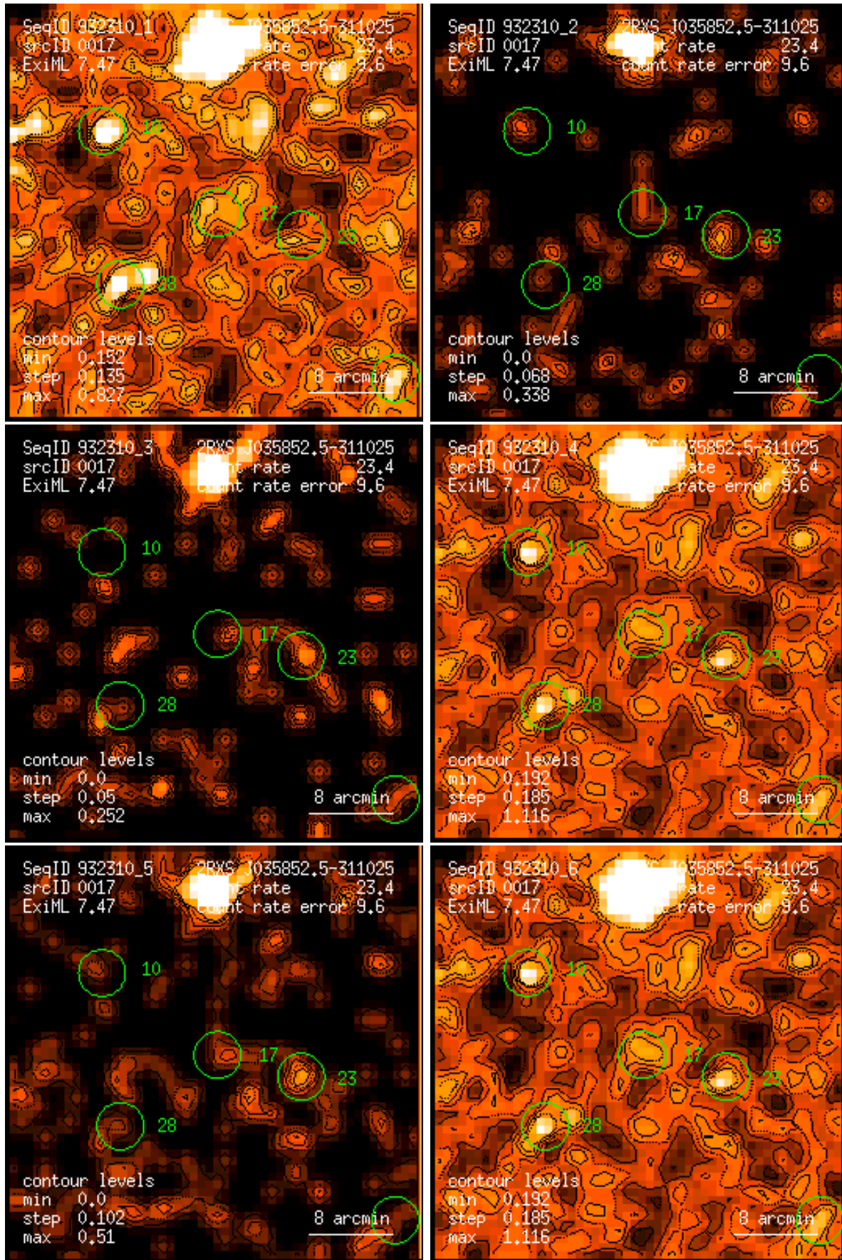
Figure 17: RASS 932310: detection 0017: band rate images, Gaussian filter: (1) PSPC channels 11 – 41, (2) 52 – 90, (3) 91 – 201, (4) 11 – 235, (5) 52 – 201, (6) 11 – 201. Broad band rates in counts/ks. Band rate contour levels in counts/ks/arcmin 2 .
