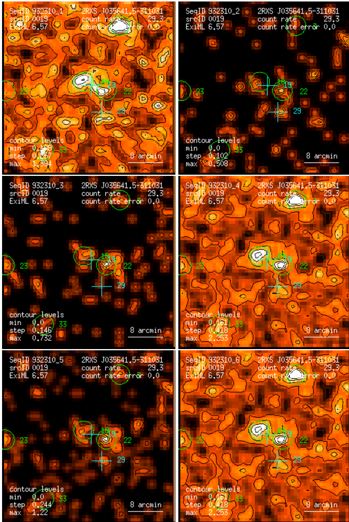
Figure 19: RASS 932310: detection 0019: band rate images, Gaussian filter: (1) PSPC channels 11 – 41, (2) 52 – 90, (3) 91 – 201, (4) 11 – 235, (5) 52 – 201, (6) 11 – 201. Broad band rates in counts/ks. Band rate contour levels in counts/ks/arcmin 2 .
