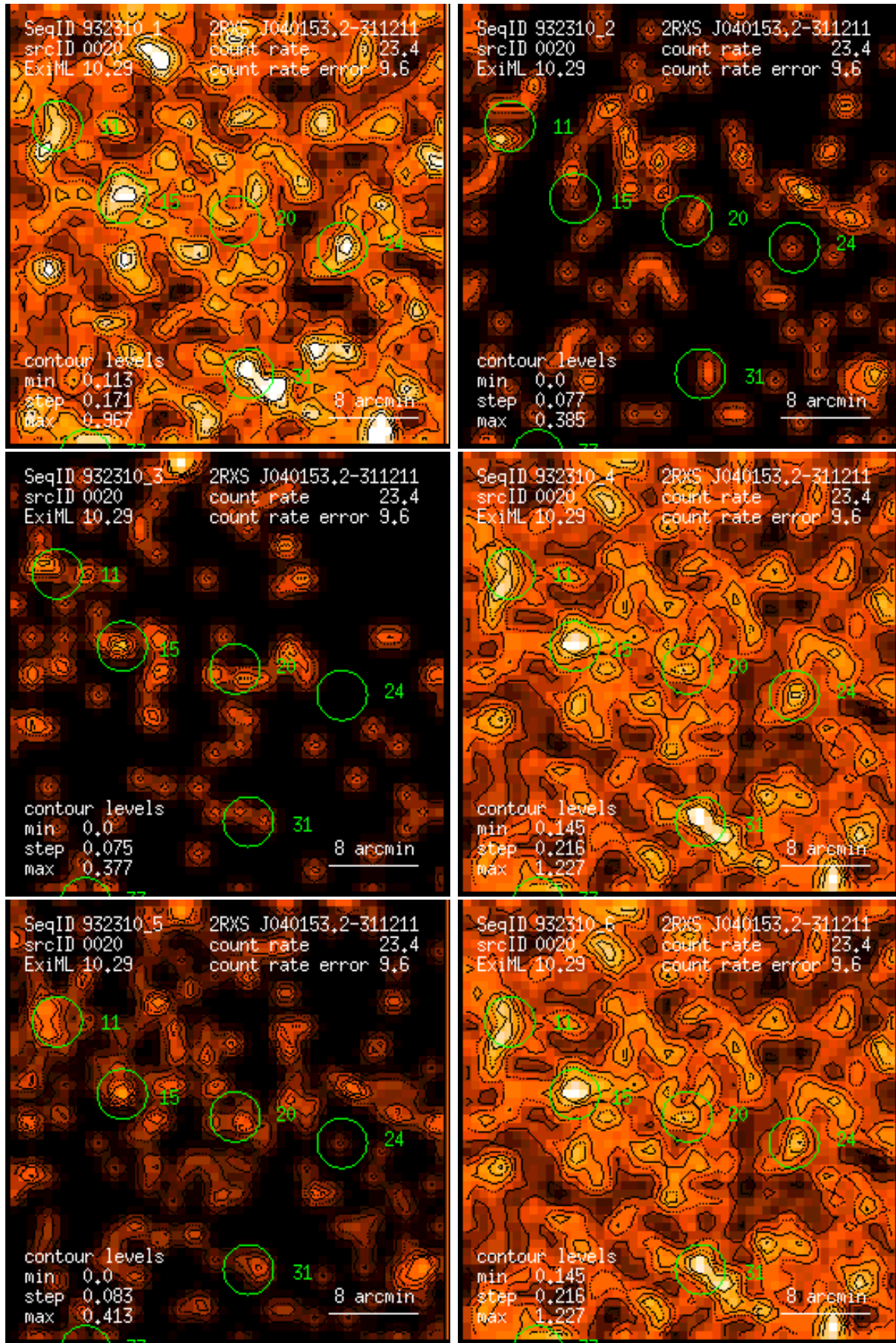
Figure 20: RASS 932310: detection 0020: band rate images, Gaussian filter: (1) PSPC channels 11 – 41, (2) 52 – 90, (3) 91 – 201, (4) 11 – 235, (5) 52 – 201, (6) 11 – 201. Broad band rates in counts/ks. Band rate contour levels in counts/ks/arcmin 2 .
