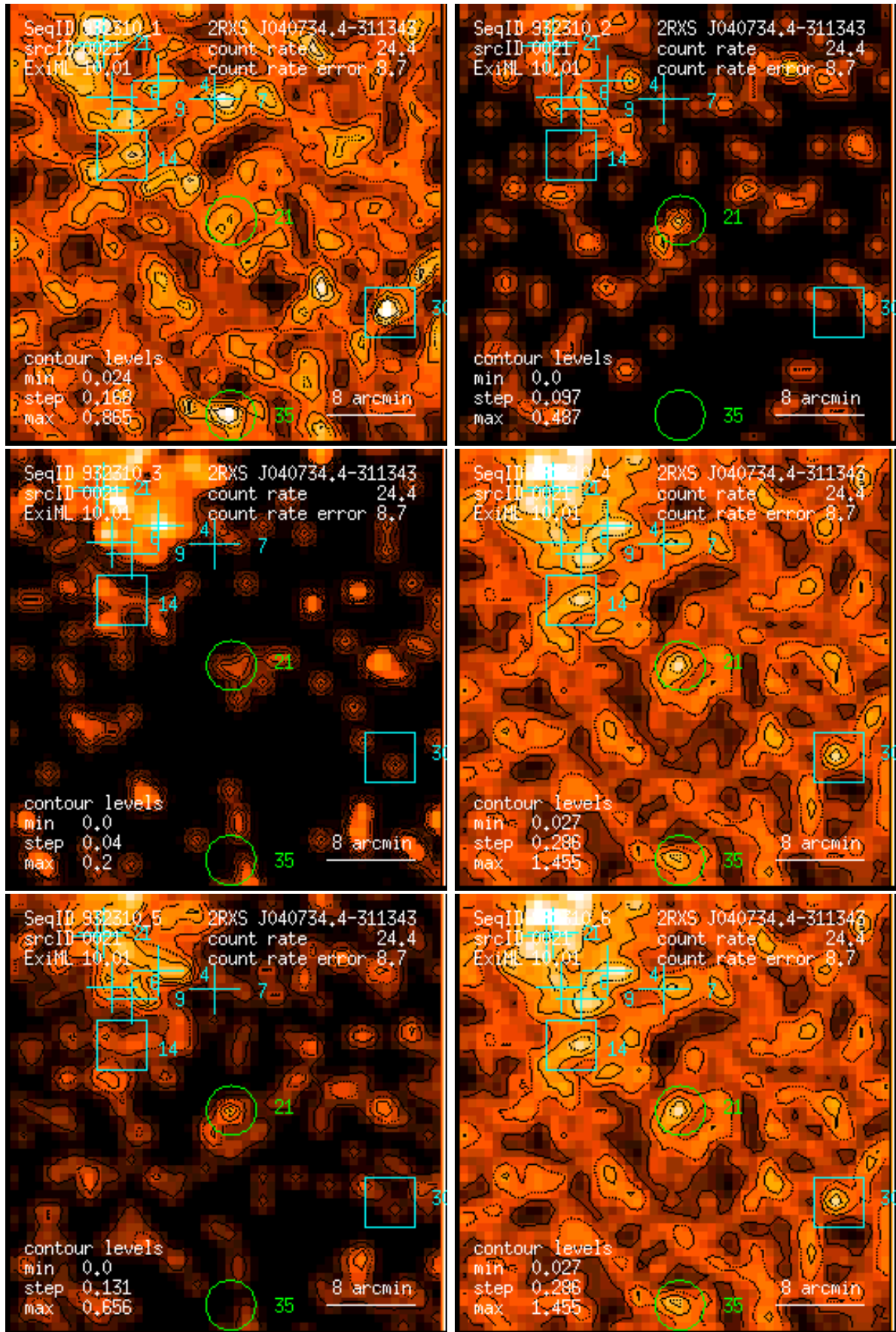
Figure 21: RASS 932310: detection 0021: band rate images, Gaussian filter: (1) PSPC channels 11 – 41, (2) 52 – 90, (3) 91 – 201, (4) 11 – 235, (5) 52 – 201, (6) 11 – 201. Broad band rates in counts/ks. Band rate contour levels in counts/ks/arcmin 2 .
