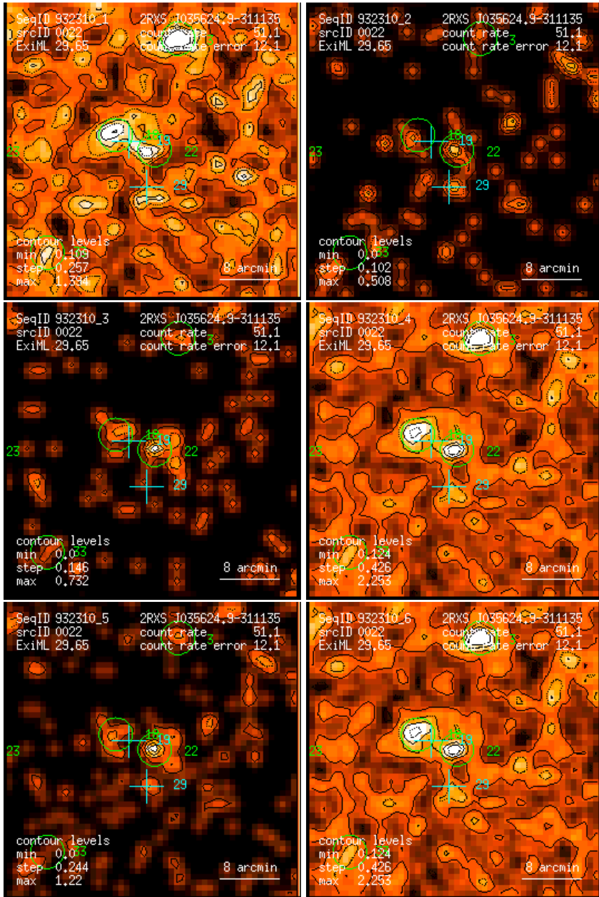
Figure 22: RASS 932310: detection 0022: band rate images, Gaussian filter: (1) PSPC channels 11 – 41, (2) 52 – 90, (3) 91 – 201, (4) 11 – 235, (5) 52 – 201, (6) 11 – 201. Broad band rates in counts/ks. Band rate contour levels in counts/ks/arcmin 2 .
