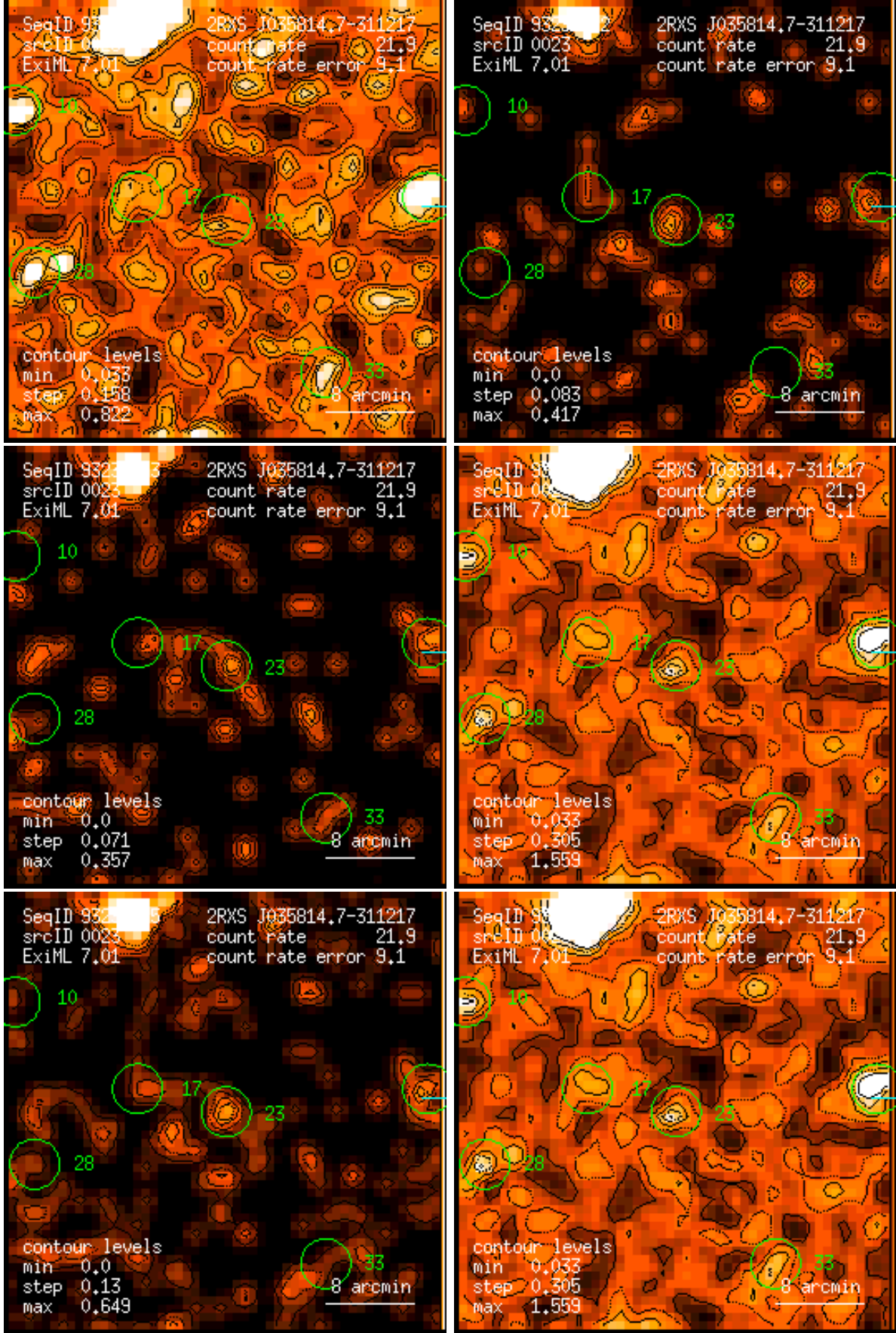
Figure 23: RASS 932310: detection 0023: band rate images, Gaussian filter: (1) PSPC channels 11 – 41, (2) 52 – 90, (3) 91 – 201, (4) 11 – 235, (5) 52 – 201, (6) 11 – 201. Broad band rates in counts/ks. Band rate contour levels in counts/ks/arcmin 2 .
