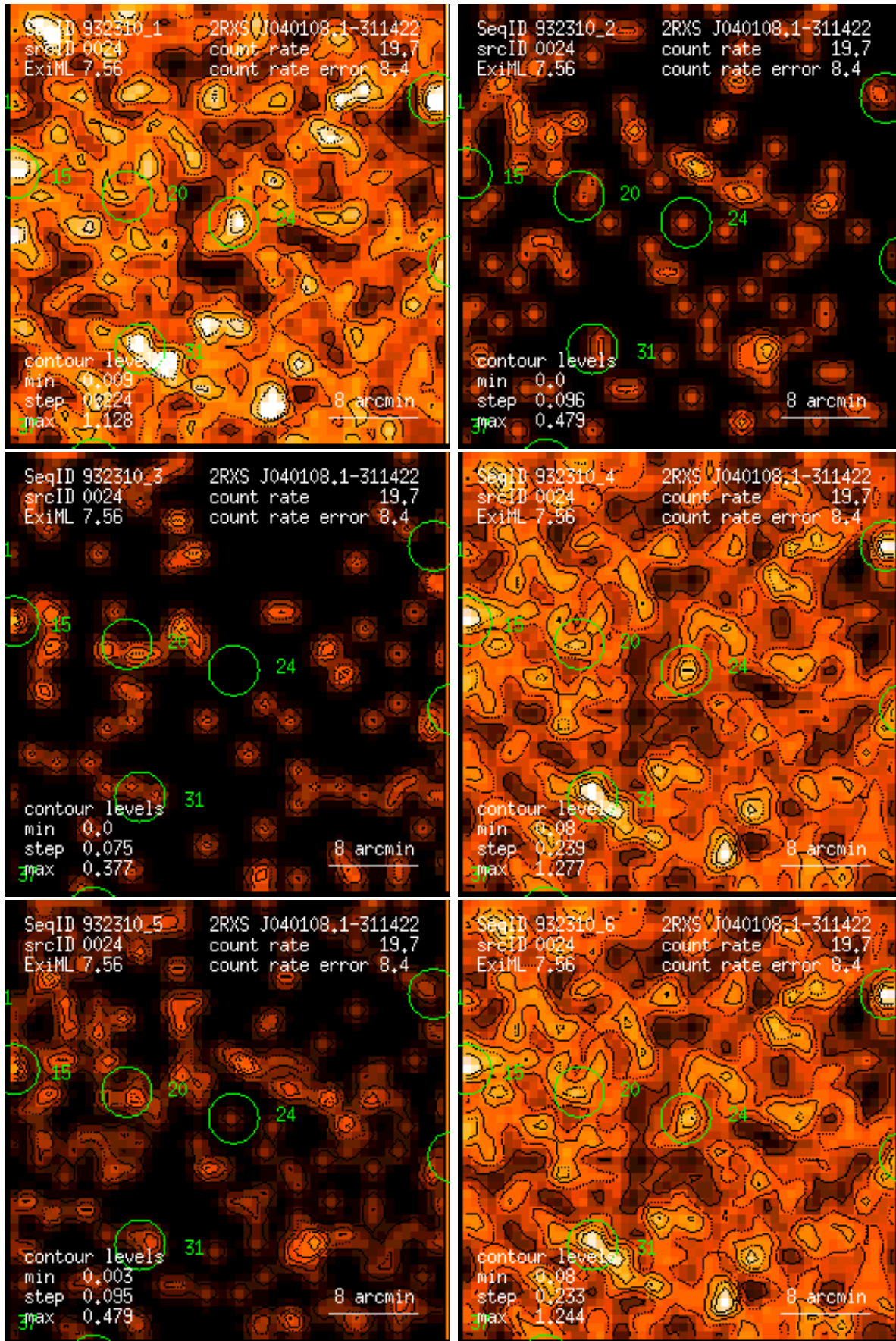
Figure 24: RASS 932310: detection 0024: band rate images, Gaussian filter: (1) PSPC channels 11 – 41, (2) 52 – 90, (3) 91 – 201, (4) 11 – 235, (5) 52 – 201, (6) 11 – 201. Broad band rates in counts/ks. Band rate contour levels in counts/ks/arcmin 2 .
