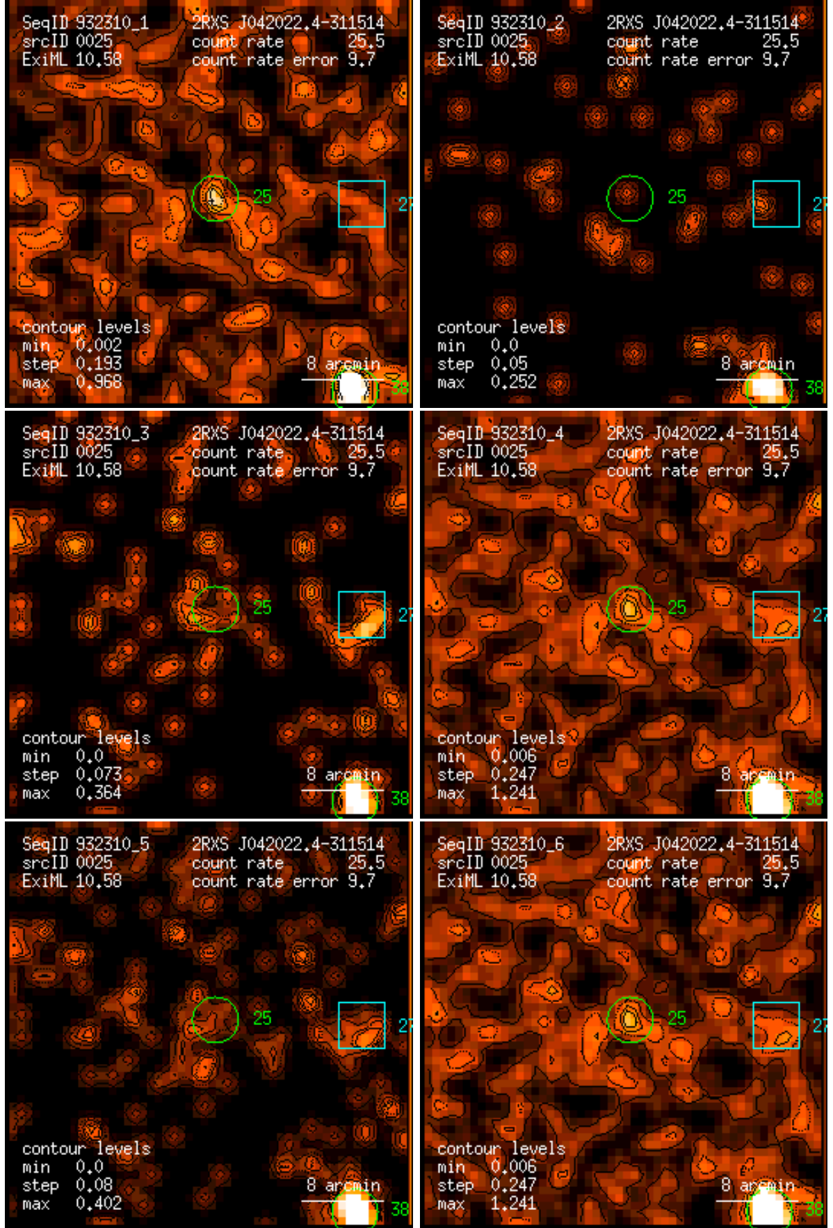
Figure 25: RASS 932310: detection 0025: band rate images, Gaussian filter: (1) PSPC channels 11 – 41, (2) 52 – 90, (3) 91 – 201, (4) 11 – 235, (5) 52 – 201, (6) 11 – 201. Broad band rates in counts/ks. Band rate contour levels in counts/ks/arcmin 2 .
