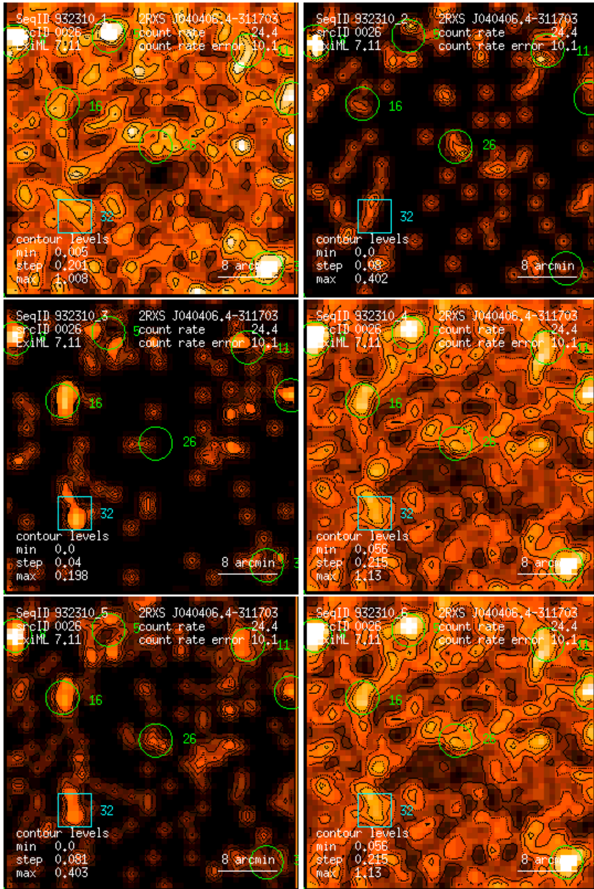
Figure 26: RASS 932310: detection 0026: band rate images, Gaussian filter: (1) PSPC channels 11 – 41, (2) 52 – 90, (3) 91 – 201, (4) 11 – 235, (5) 52 – 201, (6) 11 – 201. Broad band rates in counts/ks. Band rate contour levels in counts/ks/arcmin 2 .
