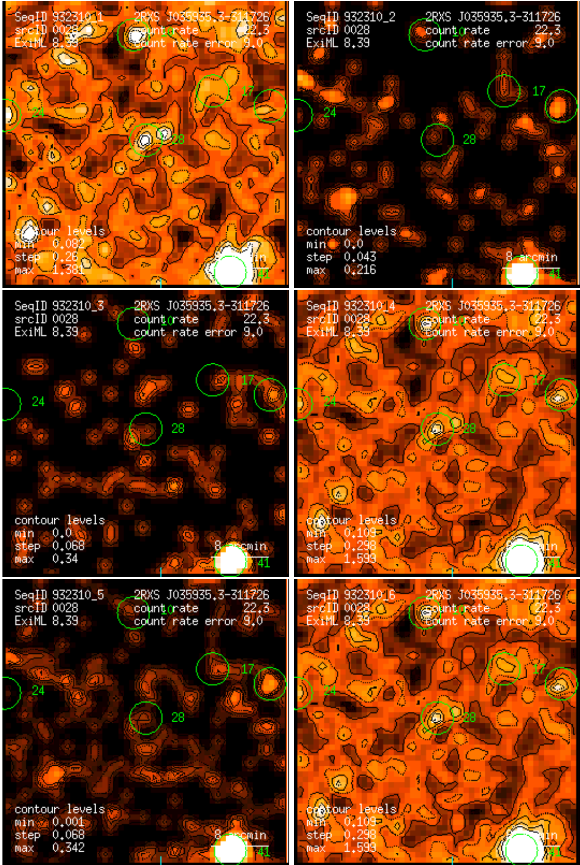
Figure 28: RASS 932310: detection 0028: band rate images, Gaussian filter: (1) PSPC channels 11 – 41, (2) 52 – 90, (3) 91 – 201, (4) 11 – 235, (5) 52 – 201, (6) 11 – 201. Broad band rates in counts/ks. Band rate contour levels in counts/ks/arcmin 2 .
