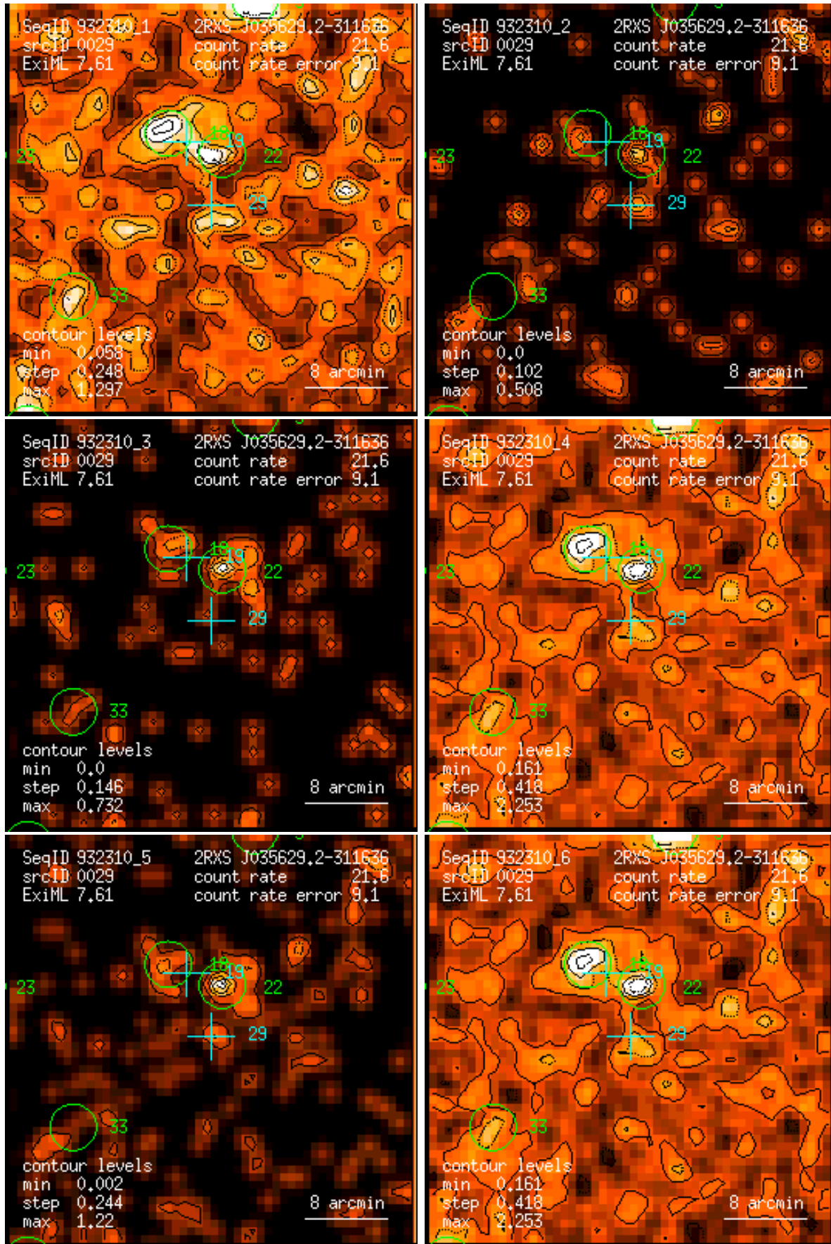
Figure 29: RASS 932310: detection 0029: band rate images, Gaussian filter: (1) PSPC channels 11 – 41, (2) 52 – 90, (3) 91 – 201, (4) 11 – 235, (5) 52 – 201, (6) 11 – 201. Broad band rates in counts/ks. Band rate contour levels in counts/ks/arcmin 2 .
