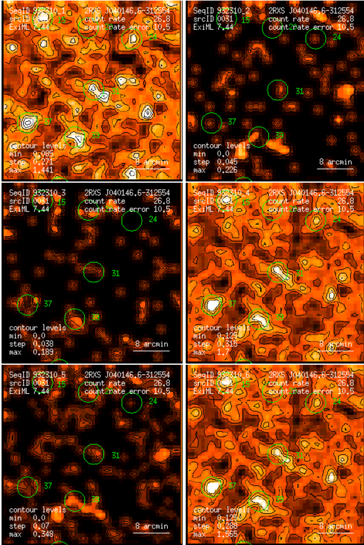
Figure 31: RASS 932310: detection 0031: band rate images, Gaussian filter: (1) PSPC channels 11 – 41, (2) 52 – 90, (3) 91 – 201, (4) 11 – 235, (5) 52 – 201, (6) 11 – 201. Broad band rates in counts/ks. Band rate contour levels in counts/ks/arcmin 2 .
