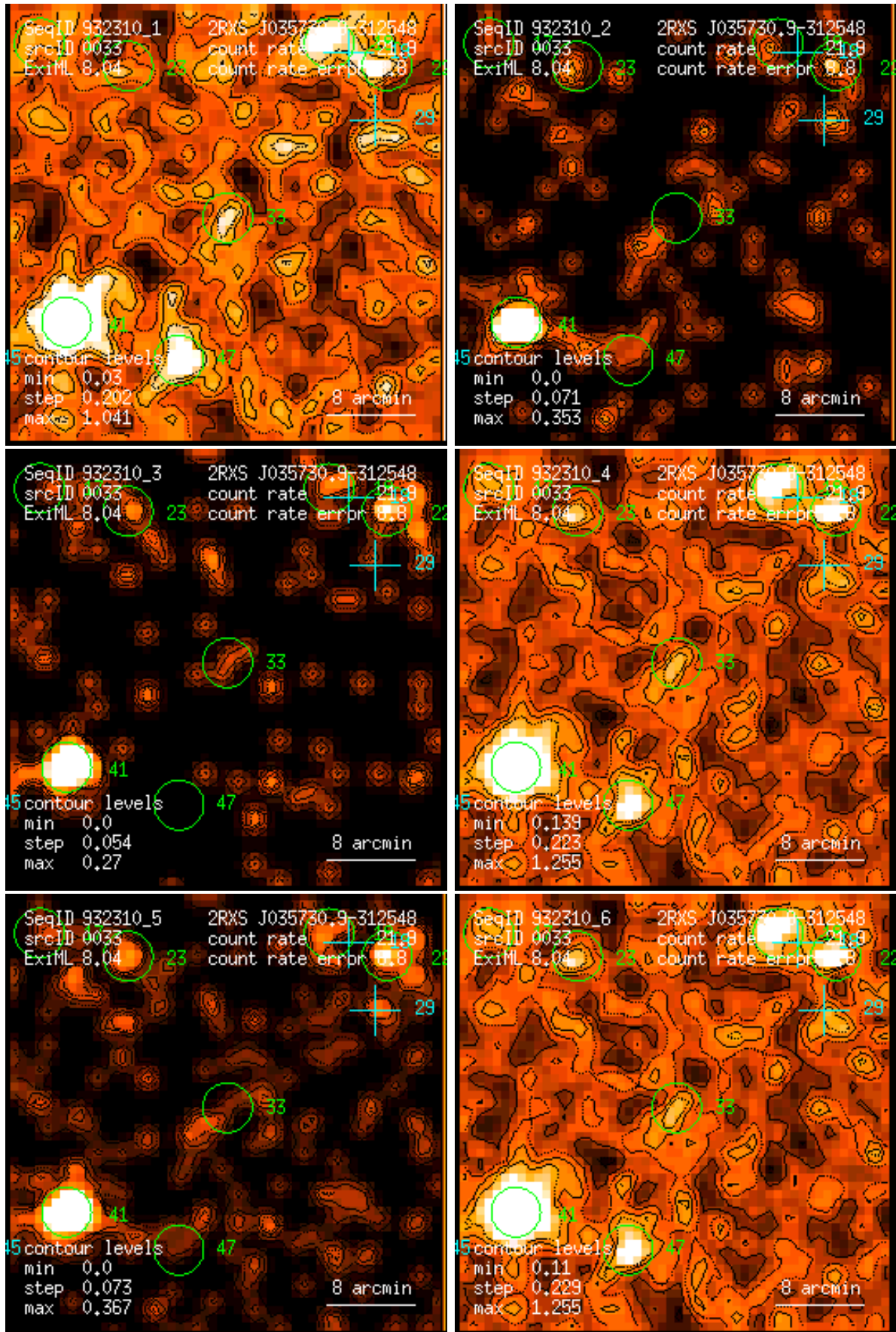
Figure 33: RASS 932310: detection 0033: band rate images, Gaussian filter: (1) PSPC channels 11 – 41, (2) 52 – 90, (3) 91 – 201, (4) 11 – 235, (5) 52 – 201, (6) 11 – 201. Broad band rates in counts/ks. Band rate contour levels in counts/ks/arcmin 2 .
