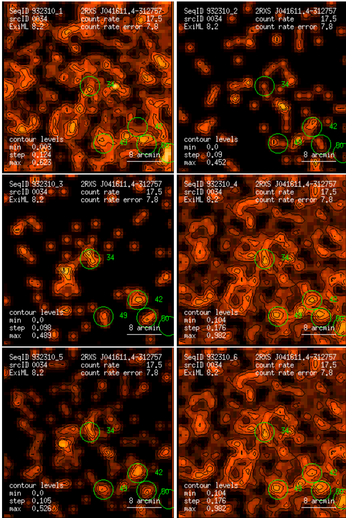
Figure 34: RASS 932310: detection 0034: band rate images, Gaussian filter: (1) PSPC channels 11 – 41, (2) 52 – 90, (3) 91 – 201, (4) 11 – 235, (5) 52 – 201, (6) 11 – 201. Broad band rates in counts/ks. Band rate contour levels in counts/ks/arcmin 2 .
