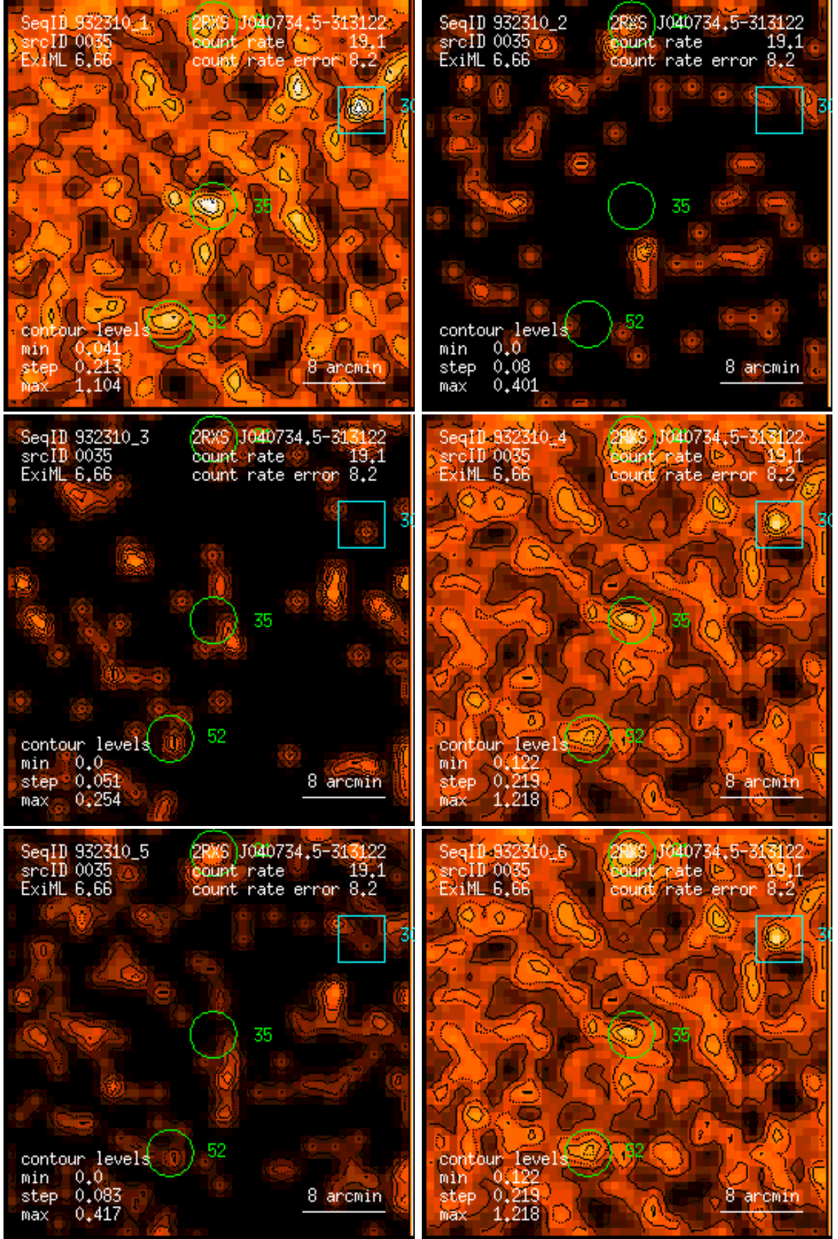
Figure 35: RASS 932310: detection 0035: band rate images, Gaussian filter: (1) PSPC channels 11 – 41, (2) 52 – 90, (3) 91 – 201, (4) 11 – 235, (5) 52 – 201, (6) 11 – 201. Broad band rates in counts/ks. Band rate contour levels in counts/ks/arcmin 2 .
