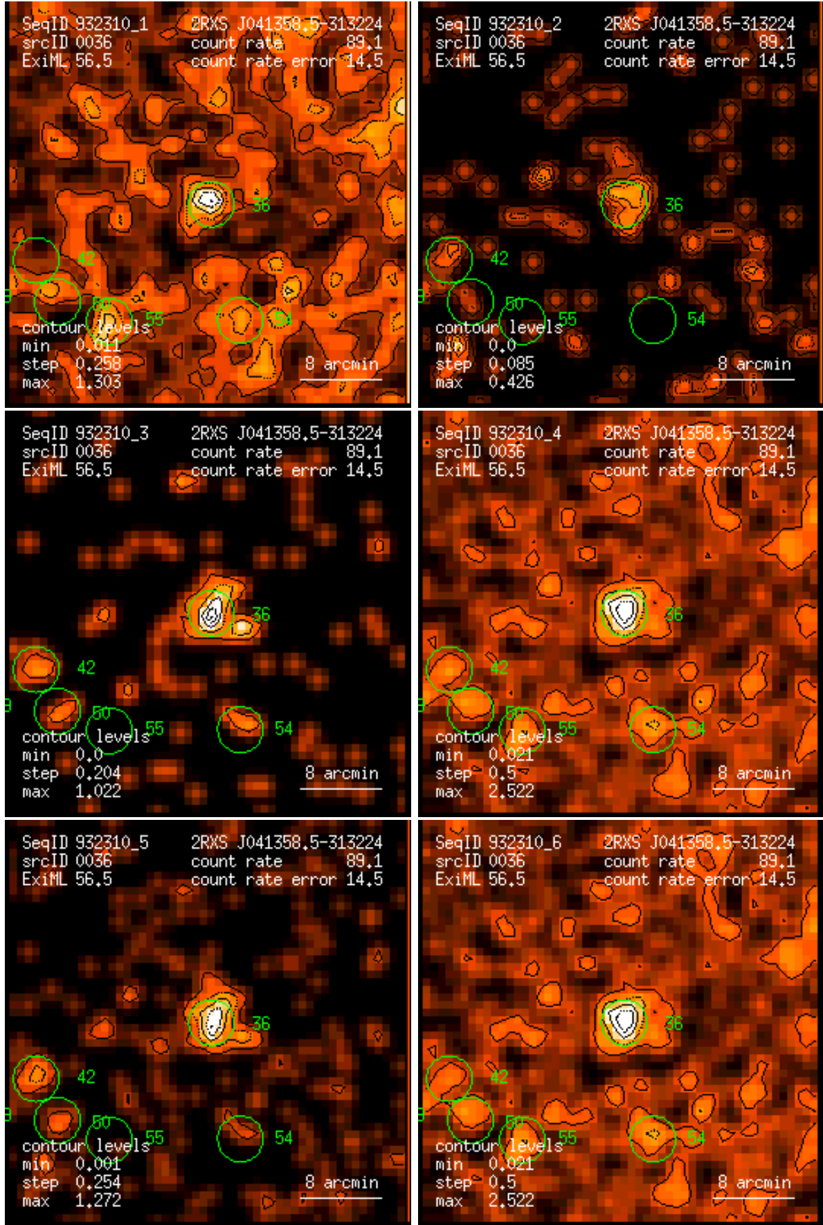
Figure 36: RASS 932310: detection 0036: band rate images, Gaussian filter: (1) PSPC channels 11 – 41, (2) 52 – 90, (3) 91 – 201, (4) 11 – 235, (5) 52 – 201, (6) 11 – 201. Broad band rates in counts/ks. Band rate contour levels in counts/ks/arcmin 2 .
