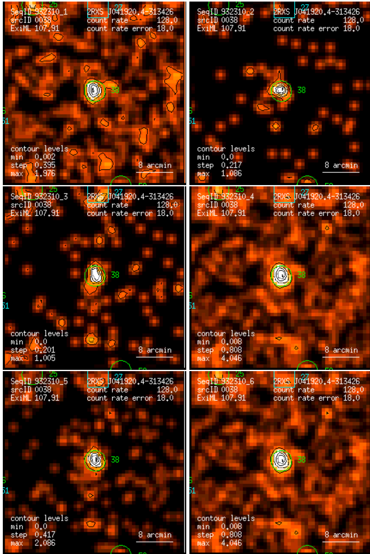
Figure 38: RASS 932310: detection 0038: band rate images, Gaussian filter: (1) PSPC channels 11 – 41, (2) 52 – 90, (3) 91 – 201, (4) 11 – 235, (5) 52 – 201, (6) 11 – 201. Broad band rates in counts/ks. Band rate contour levels in counts/ks/arcmin 2 .
