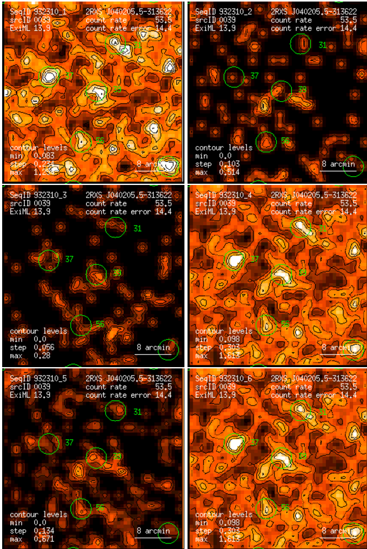
Figure 39: RASS 932310: detection 0039: band rate images, Gaussian filter: (1) PSPC channels 11 – 41, (2) 52 – 90, (3) 91 – 201, (4) 11 – 235, (5) 52 – 201, (6) 11 – 201. Broad band rates in counts/ks. Band rate contour levels in counts/ks/arcmin 2 .
