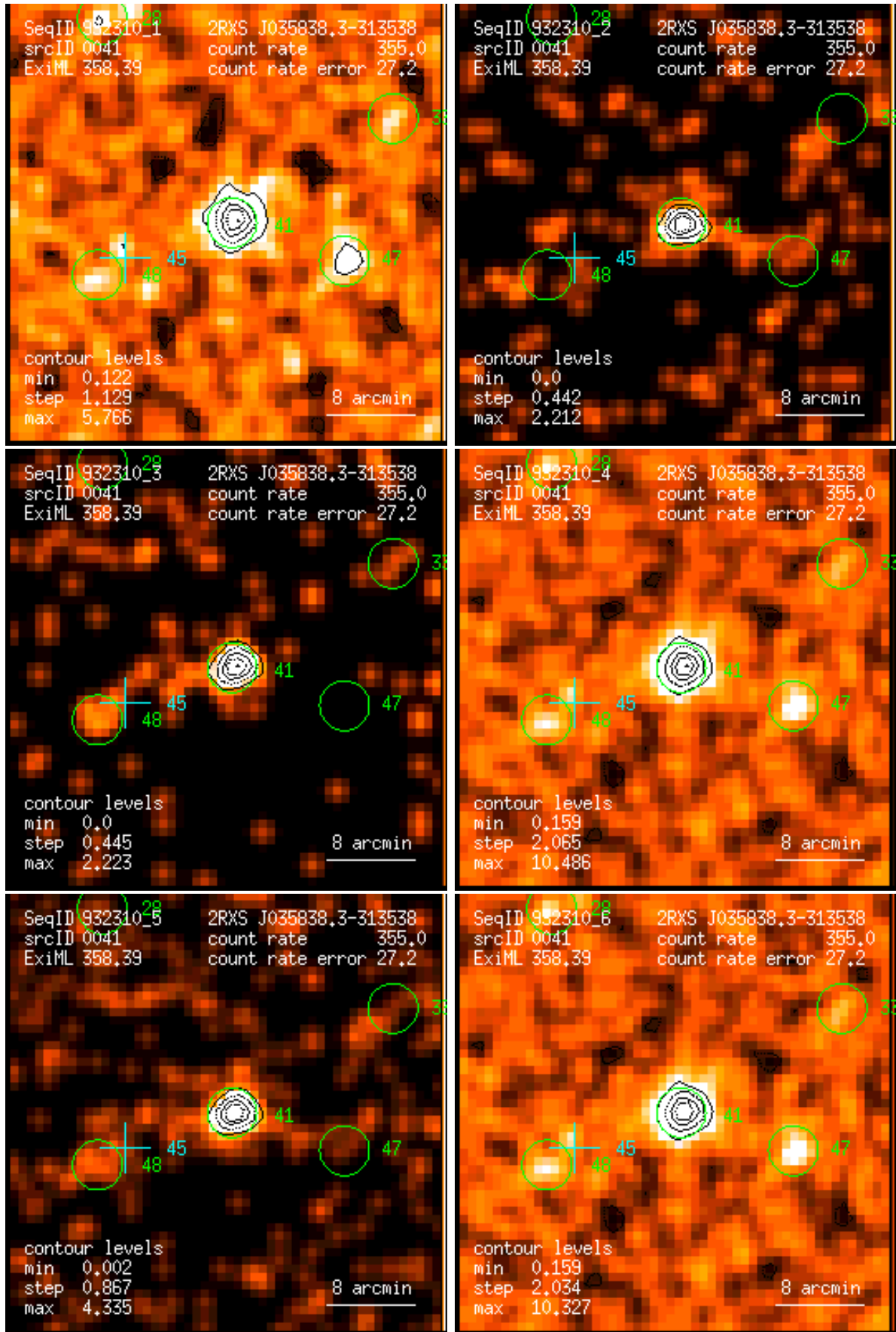
Figure 41: RASS 932310: detection 0041: band rate images, Gaussian filter: (1) PSPC channels 11 – 41, (2) 52 – 90, (3) 91 – 201, (4) 11 – 235, (5) 52 – 201, (6) 11 – 201. Broad band rates in counts/ks. Band rate contour levels in counts/ks/arcmin 2 .
