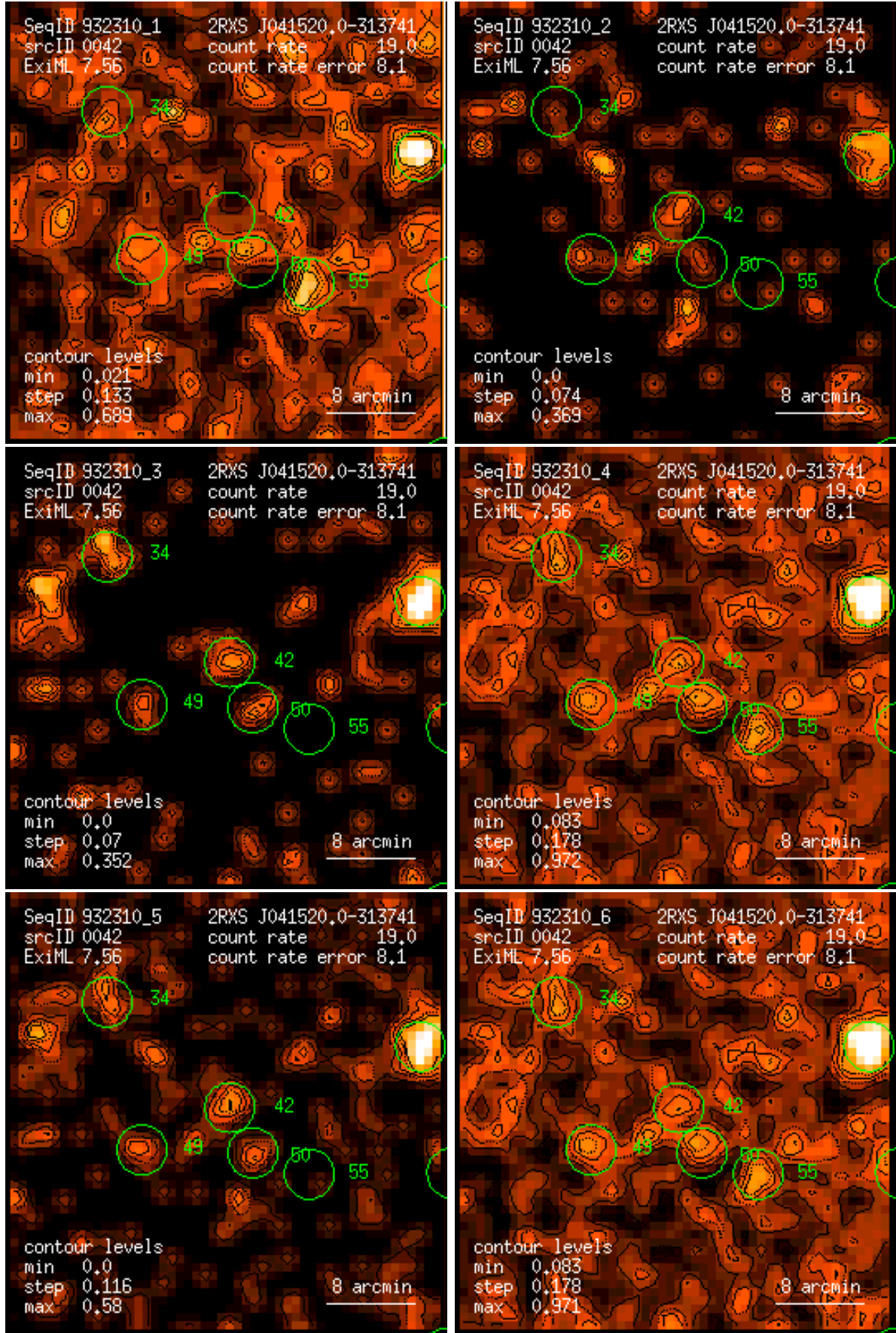
Figure 42: RASS 932310: detection 0042: band rate images, Gaussian filter: (1) PSPC channels 11 – 41, (2) 52 – 90, (3) 91 – 201, (4) 11 – 235, (5) 52 – 201, (6) 11 – 201. Broad band rates in counts/ks. Band rate contour levels in counts/ks/arcmin 2 .
