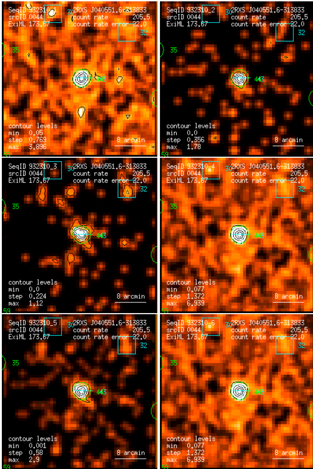
Figure 44: RASS 932310: detection 0044: band rate images, Gaussian filter: (1) PSPC channels 11 – 41, (2) 52 – 90, (3) 91 – 201, (4) 11 – 235, (5) 52 – 201, (6) 11 – 201. Broad band rates in counts/ks. Band rate contour levels in counts/ks/arcmin 2 .
