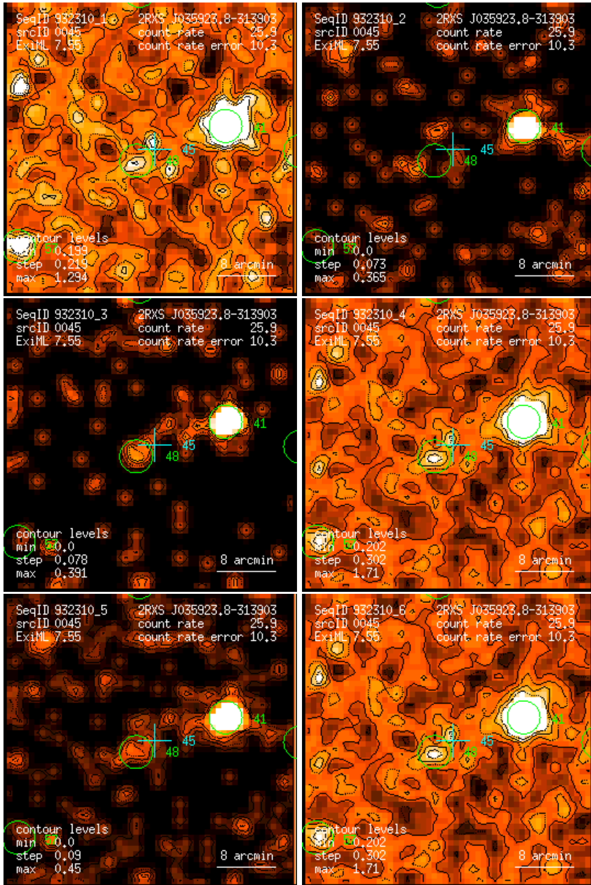
Figure 45: RASS 932310: detection 0045: band rate images, Gaussian filter: (1) PSPC channels 11 – 41, (2) 52 – 90, (3) 91 – 201, (4) 11 – 235, (5) 52 – 201, (6) 11 – 201. Broad band rates in counts/ks. Band rate contour levels in counts/ks/arcmin 2 .
