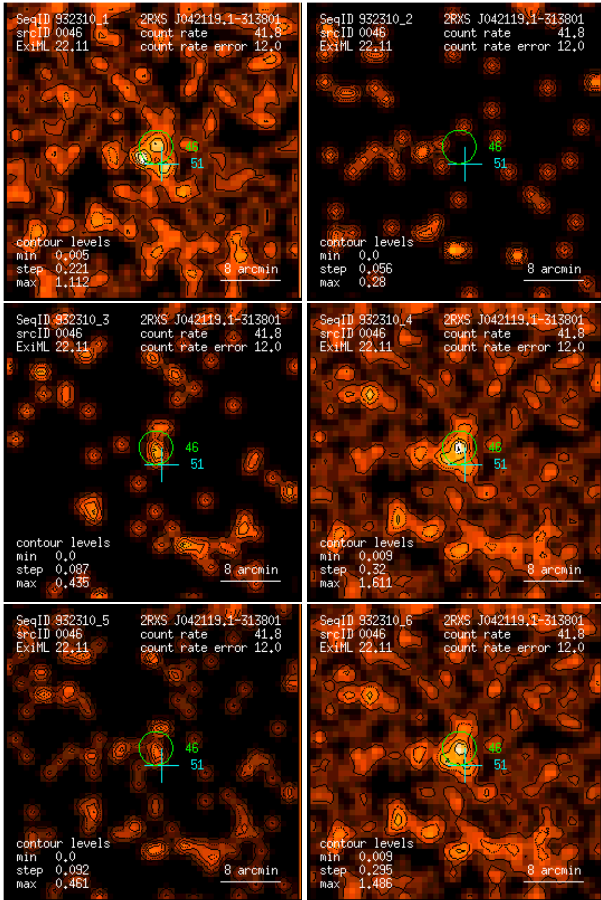
Figure 46: RASS 932310: detection 0046: band rate images, Gaussian filter: (1) PSPC channels 11 – 41, (2) 52 – 90, (3) 91 – 201, (4) 11 – 235, (5) 52 – 201, (6) 11 – 201. Broad band rates in counts/ks. Band rate contour levels in counts/ks/arcmin 2 .
