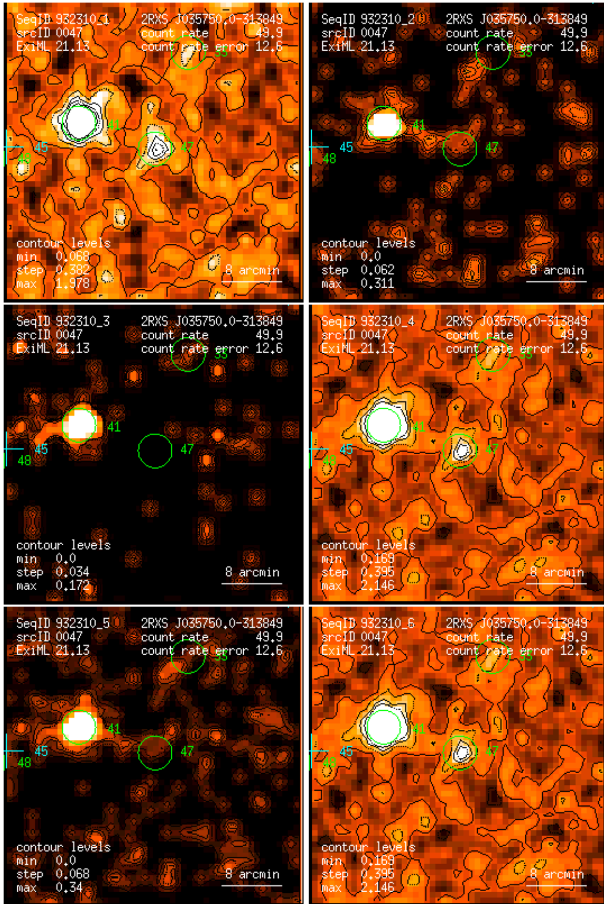
Figure 47: RASS 932310: detection 0047: band rate images, Gaussian filter: (1) PSPC channels 11 – 41, (2) 52 – 90, (3) 91 – 201, (4) 11 – 235, (5) 52 – 201, (6) 11 – 201. Broad band rates in counts/ks. Band rate contour levels in counts/ks/arcmin 2 .
