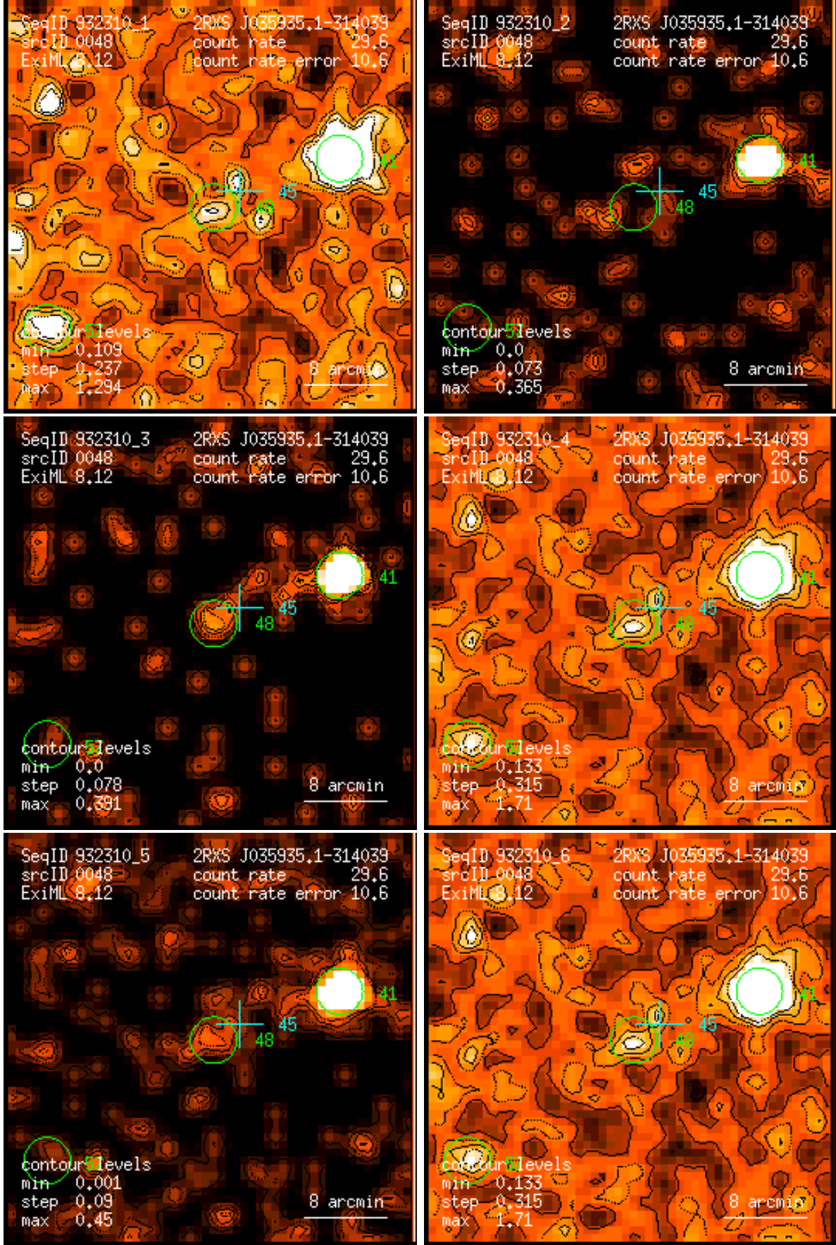
Figure 48: RASS 932310: detection 0048: band rate images, Gaussian filter: (1) PSPC channels 11 – 41, (2) 52 – 90, (3) 91 – 201, (4) 11 – 235, (5) 52 – 201, (6) 11 – 201. Broad band rates in counts/ks. Band rate contour levels in counts/ks/arcmin 2 .
