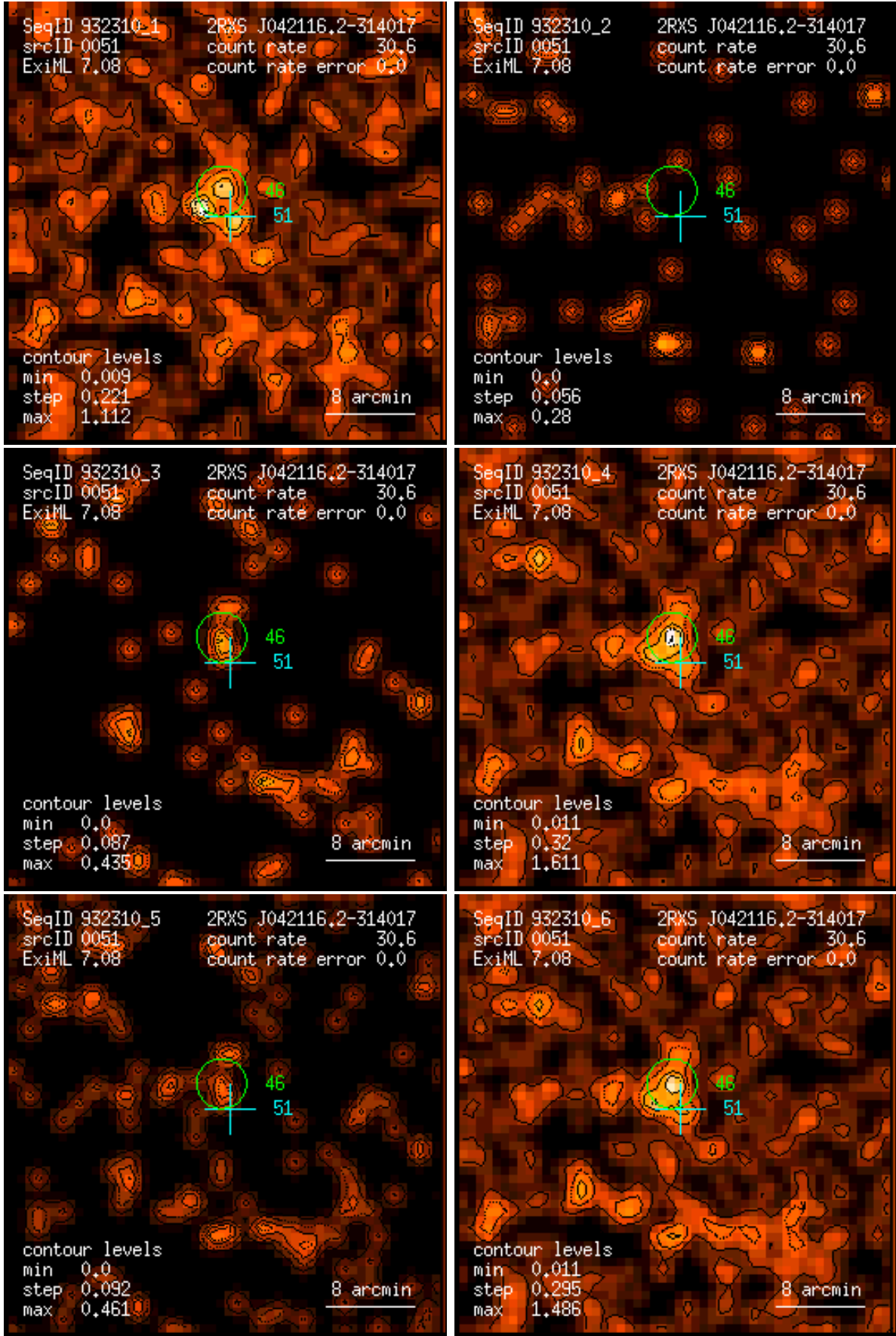
Figure 51: RASS 932310: detection 0051: band rate images, Gaussian filter: (1) PSPC channels 11 – 41, (2) 52 – 90, (3) 91 – 201, (4) 11 – 235, (5) 52 – 201, (6) 11 – 201. Broad band rates in counts/ks. Band rate contour levels in counts/ks/arcmin 2 .
