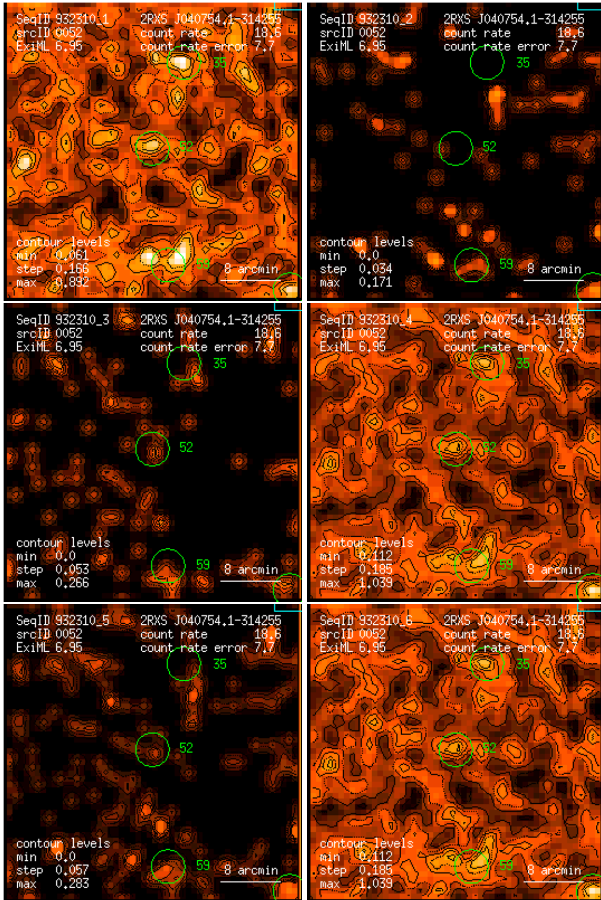
Figure 52: RASS 932310: detection 0052: band rate images, Gaussian filter: (1) PSPC channels 11 – 41, (2) 52 – 90, (3) 91 – 201, (4) 11 – 235, (5) 52 – 201, (6) 11 – 201. Broad band rates in counts/ks. Band rate contour levels in counts/ks/arcmin 2 .
