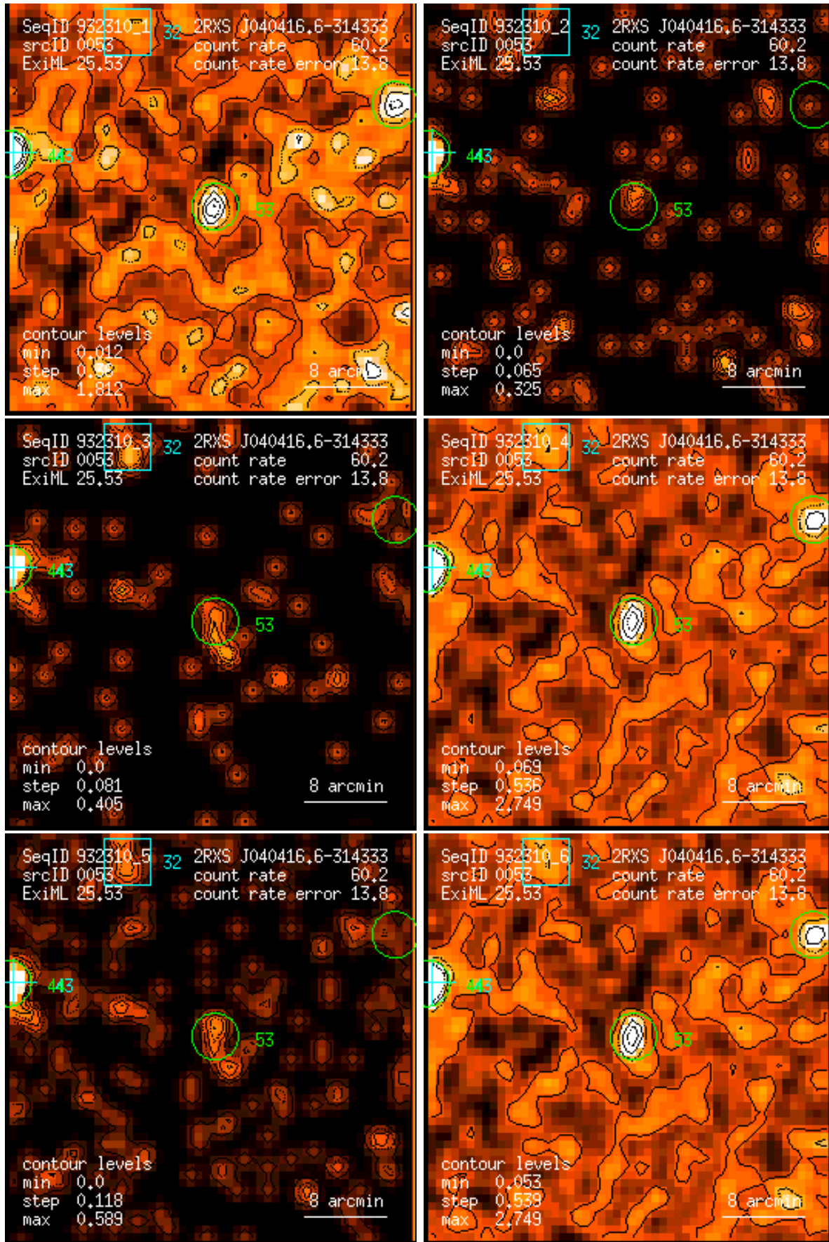
Figure 53: RASS 932310: detection 0053: band rate images, Gaussian filter: (1) PSPC channels 11 – 41, (2) 52 – 90, (3) 91 – 201, (4) 11 – 235, (5) 52 – 201, (6) 11 – 201. Broad band rates in counts/ks. Band rate contour levels in counts/ks/arcmin 2 .
