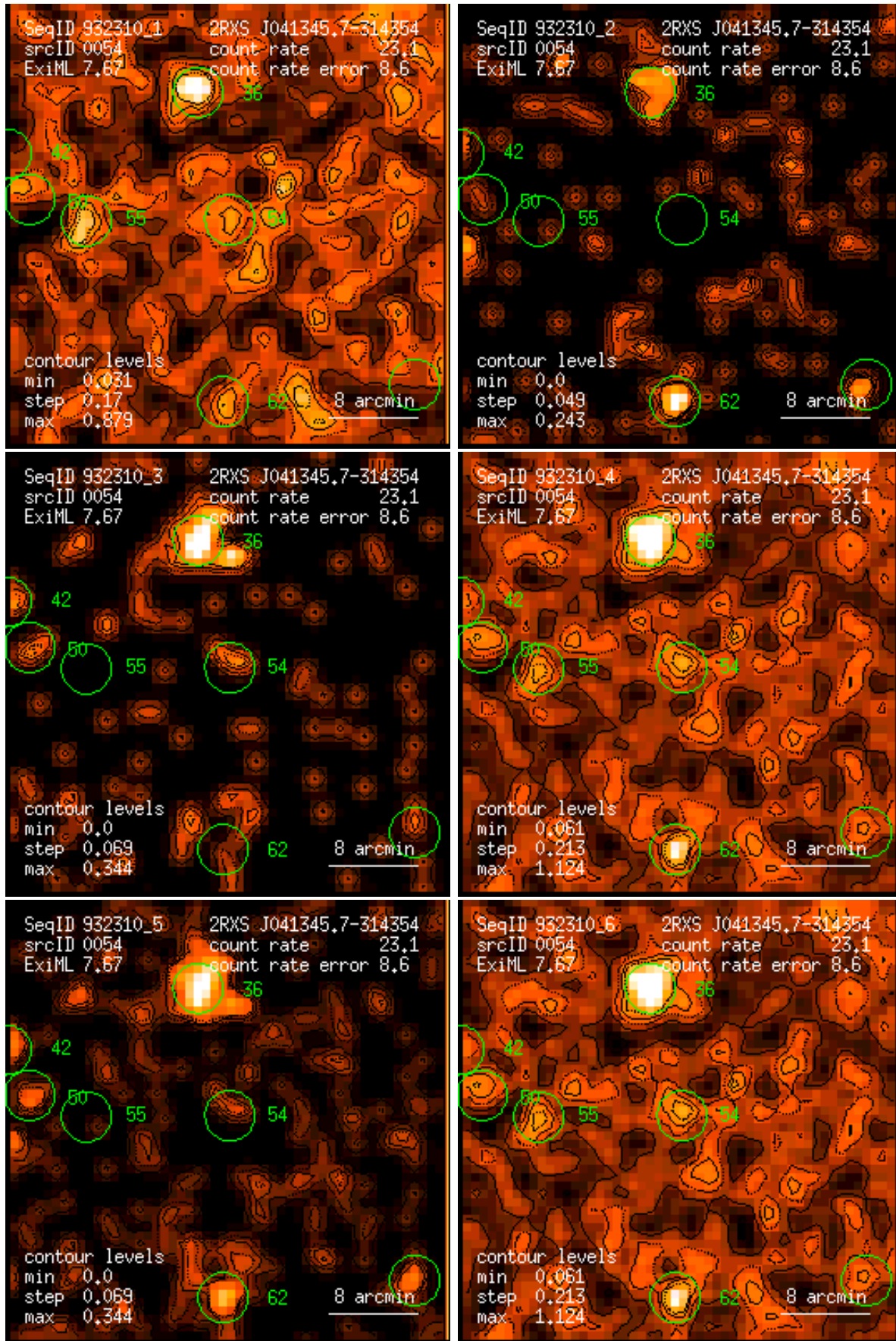
Figure 54: RASS 932310: detection 0054: band rate images, Gaussian filter: (1) PSPC channels 11 – 41, (2) 52 – 90, (3) 91 – 201, (4) 11 – 235, (5) 52 – 201, (6) 11 – 201. Broad band rates in counts/ks. Band rate contour levels in counts/ks/arcmin 2 .
