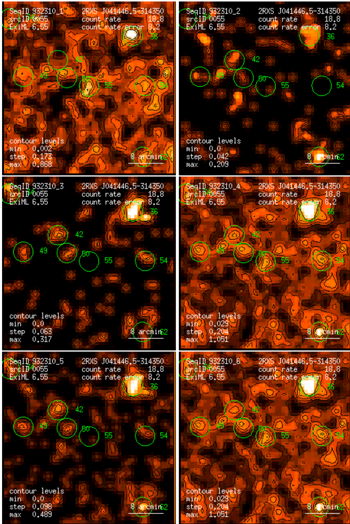
Figure 55: RASS 932310: detection 0055: band rate images, Gaussian filter: (1) PSPC channels 11 – 41, (2) 52 – 90, (3) 91 – 201, (4) 11 – 235, (5) 52 – 201, (6) 11 – 201. Broad band rates in counts/ks. Band rate contour levels in counts/ks/arcmin 2 .
